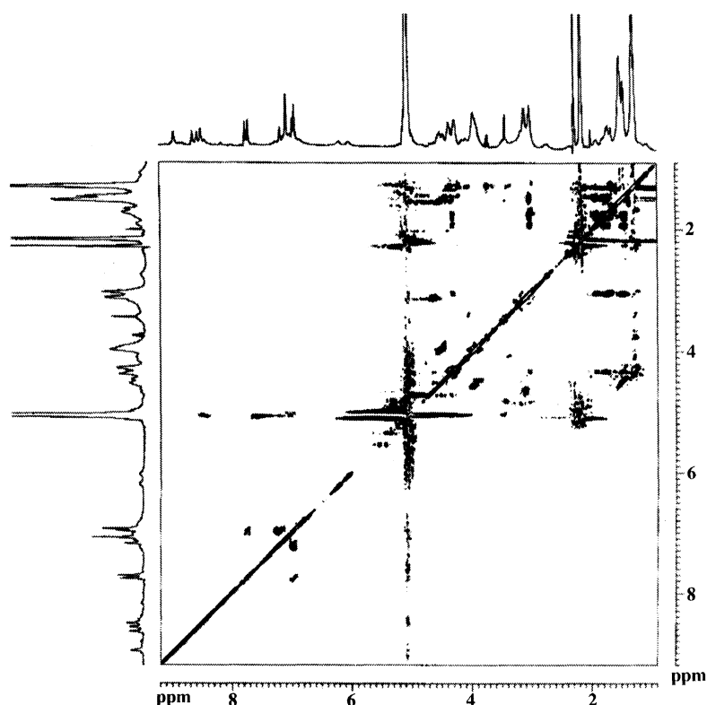
Fig. 6: TOCSY spectrum of -TASHHK- in presence of Zn(II) ions, in peptide - Zn(II) ratio 1.2:1 ( c_L = 15 mM) and \text{pH}^+ 10.3 , in D 2 O:H 2 O 1:4 mixture.
