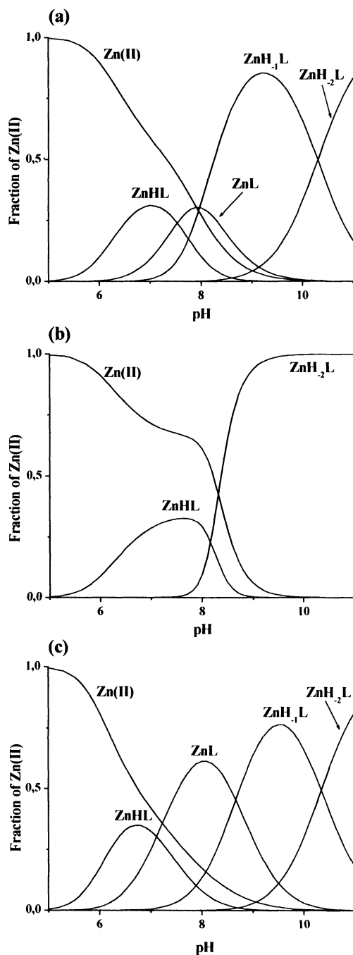
Fig. 3: Species distribution diagrams of Zn(II) complexes with (a) -TESHHK-, (b) -TASHHK- and (c) -TEAHHK- ( c_{Zn} = c_L = 1 mM, T = 25 °C, I = 0.1 M KNO_3 ).
