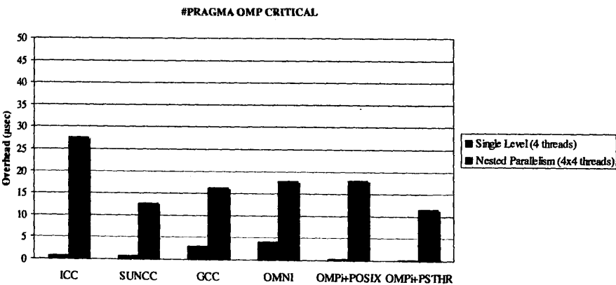
Figure 4.4: Overheads for the parallel, for, single and critical.
