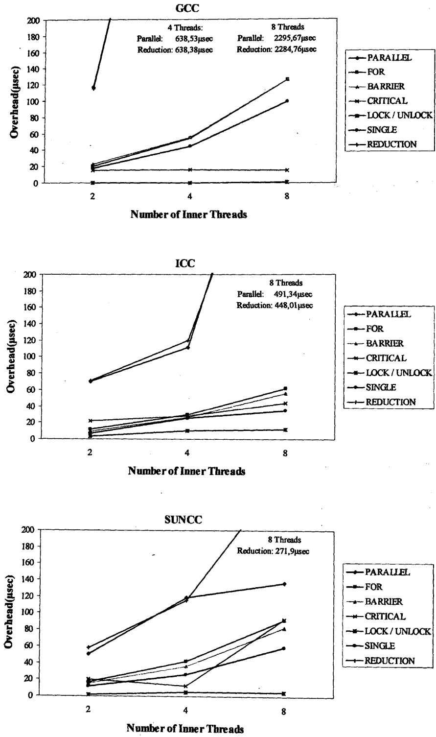
Figure 4.7: Synchronization overheads for GCC, ICC and SUNCC on a different population of threads.
