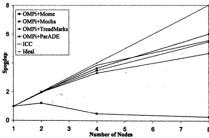
Figure 6.4: Speedups for NAS EP, MM and MD.
