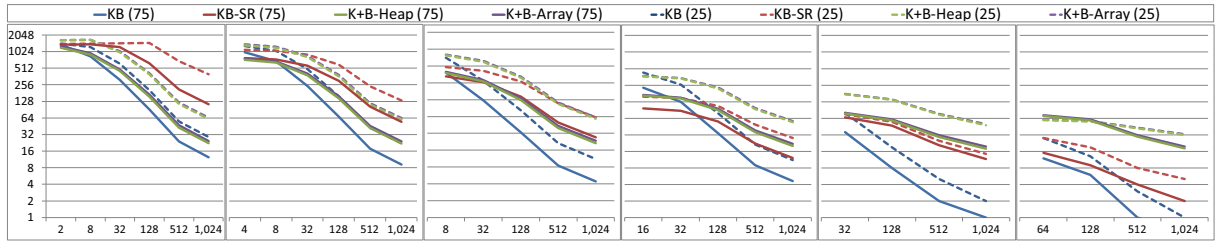
Figure 7.6: Performance evaluation in FPS ( \log_2 scale) of our bounded K^+B methods and the sorting-aware k -buffer methods for a large set of k values. Pixel density is shown in brackets.
