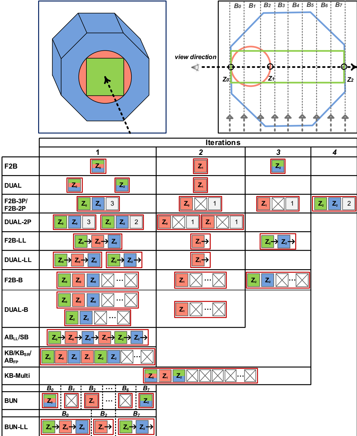
Figure 6.1: Overview of peeling results for our proposed methods and their predecessors. Z_0, Z_1 and Z_2 indicate the depth layers captured by ray casting (black dashed line) and B_0, B_1, \dots, B_7 the uniformly distributed buckets. Each column shows the produced output of each method for the corresponding iteration: extracted fragment(s) painted with the color of an object and coplanarity counters. Squares painted with more than one color demonstrate z-fighting artifacts (it is undefined which fragment might win the z-test). To distinguish between fragments of the same object, we have included their depth value to their associated square.
