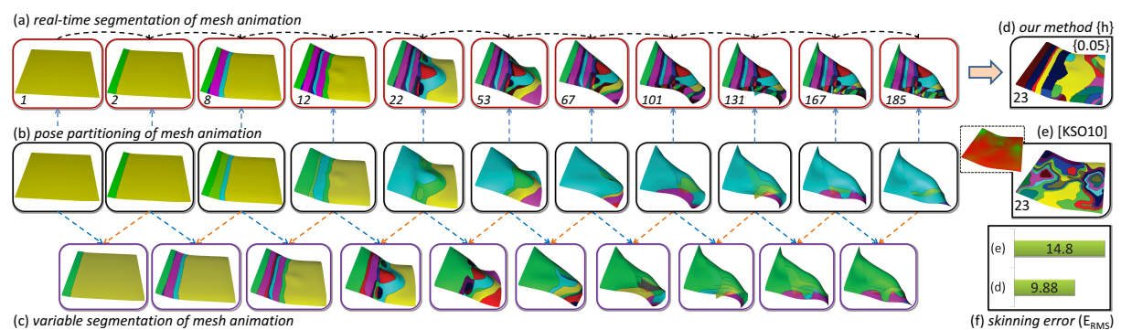
Figure 3.6: Flowing cloth mesh animation : (a) Real-time segmentation construction process. (b) Pose partitioning enhanced by our color propagation scheme. (c) Variable segmentation. (d) A snapshot of our joint segmentation which consists of 23 components. Our output is superior in the context of (f) skinning error when compared to (e) the one derived from [69] (thumbnail of the normalized feature space is also provided).
