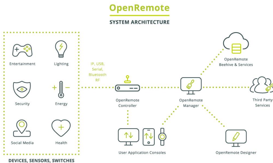
Figure 27 – The OpenRemote Platform Architecture.
