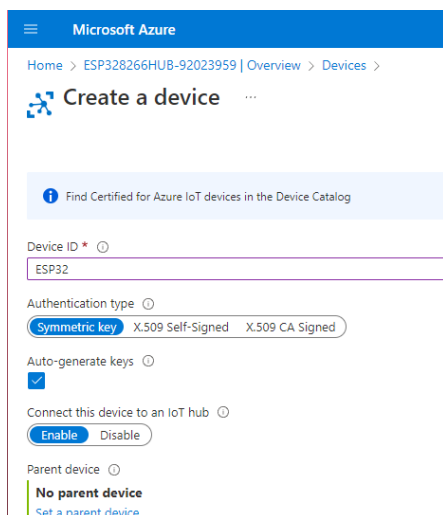
Figure 44 – Creating a device on the Azure IoT Hub.
