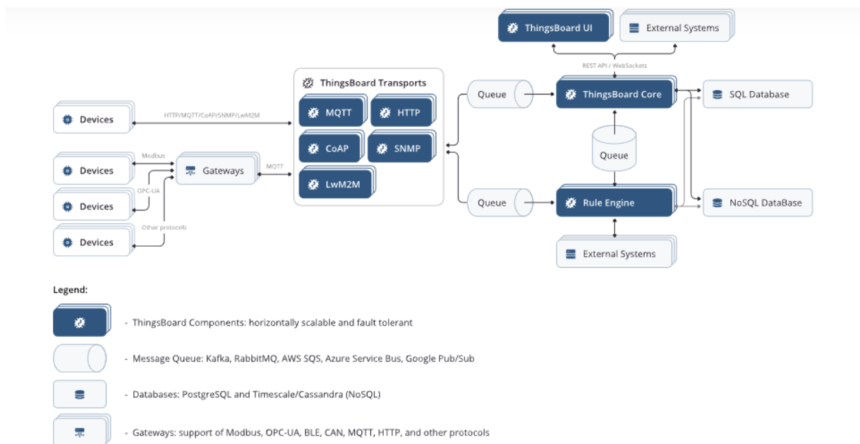
Figure 19 – The ThingsBoard architecture
