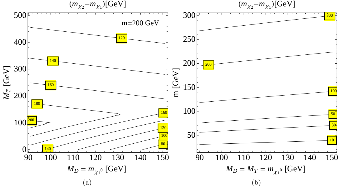
Figure 2: The mass difference, |m_{\chi_2^0}| - |m_{\chi_1^0}| , between the next-to-lightest and the lightest neutral particle state in the doublet-triplet fermionic DM model on (a) M_D vs. M_T with m = 200 GeV, and (b) on M_D vs. m with M_T = M_D , plane. For both plots and for the rest to come, it is always, m_{\chi_1^0} = M_D .
