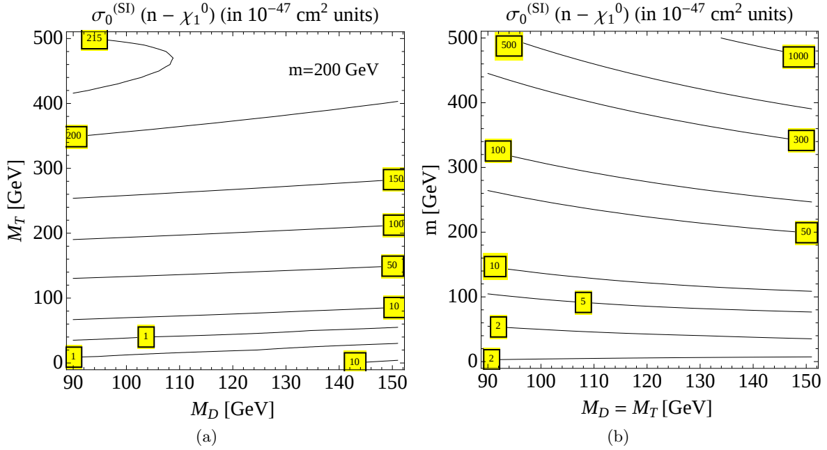
Figure 10: Results (in boxed labels) for the Spin-Independent (SI) scattering cross section for the nucleon - WIMP ( n - \chi_1^0 ) in units of 10^{-47} \text{ cm}^2 on a M_D vs. M_T plane for fixed parameter m = Yv = 200 GeV (left) and on M_D vs. m plane for fixed M_T = M_D GeV (right).
