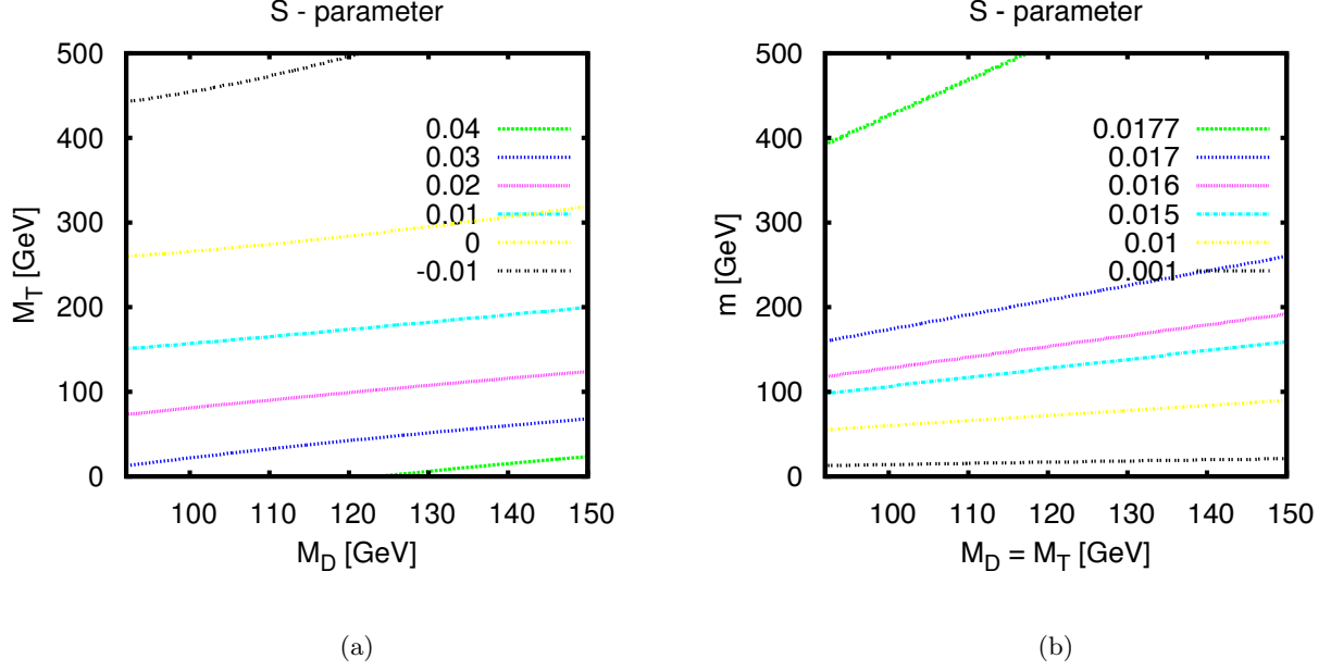
Figure 4: Contour plots of the S -parameter on the M_D vs. M_T plane (left) for m = 200 GeV and on M_D vs. m plane (right) for M_T = M_D .
