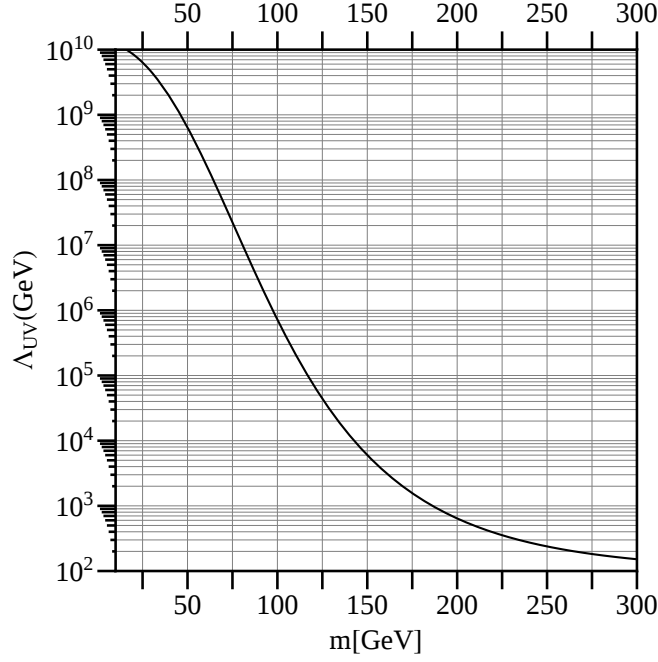
Figure 12: The vacuum stability plot: \Lambda_{UV} against m = Yv .
