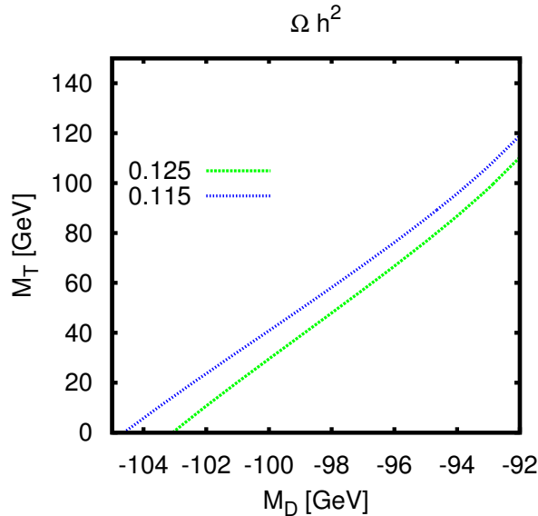
Figure 8: Same as Fig. 7a but for negative values of M_D .
