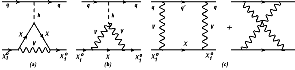
Figure 9: Feynman diagrams (in unitary gauge) related to spin independent (SI) elastic cross section \chi_1^0 + q \rightarrow \chi_1^0 + q where q = u, d, s – light quarks. Particle V represents W or Z and \chi represents \chi_{i=1..2}^\pm or \chi_{i=1..3}^0 , respectively. One loop self energy corrections are absent in the particular scenario we have chosen.
