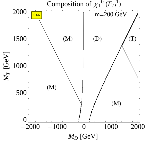
Figure 3: The composition of the WIMP in terms of (D)oublet, (T)riplet and (M)ixed states following the definition given in the paragraph below eq. (2.52), on a M_D vs. M_T plane and for fixed (common) Yukawa coupling, Y = m/v \simeq 200/174 \simeq 1.15 .
