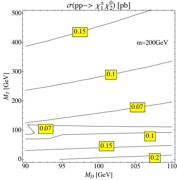
Figure 13: Contours of the production cross section for the new fermions, \sigma(pp \rightarrow \chi_1^\pm \chi_2^0) [in pb], on M_D vs. M_T plane, at LHC with \sqrt{s} = 8 TeV.
