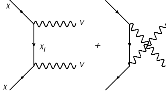
Figure 5: Lower level Feynman diagrams contributing to annihilation cross section for the process \chi + \chi \rightarrow V + V for V = W, Z .
