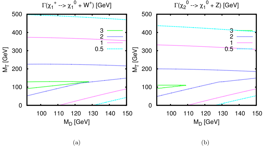
Figure 14: Contour plots for the decay rates [in GeV] for the processes \chi_1^+ \rightarrow \chi_1^0 + W^+ (left) and \chi_2^0 \rightarrow \chi_1^0 + Z (right). We assume m = 200 GeV.
