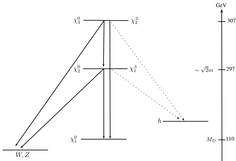
Figure 1: A sketch for the mass spectrum and decays of the new physical doublet and triplet fermions. The lightest neutral particle, \chi_1^0 is an equal admixture of the two doublets and has mass M_D . Particles \chi_2^0 ( \chi_3^0 ) and \chi_1^\pm ( \chi_2^\pm ) are mass degenerate. For the spectrum masses written to the right we have chosen M_D = 110 GeV, M_T = 100 GeV and m = Yv = 200 GeV. It provides the correct relic density abundance for dark matter [see Section 4] and is currently about \sim 10 times less sensitive to current direct detection searches [see Section 5].
