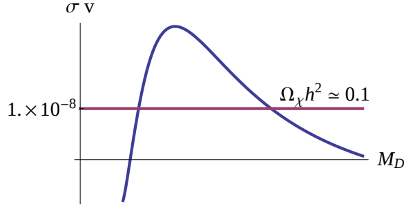
Figure 6: Sketch of the resulting annihilation cross section.
