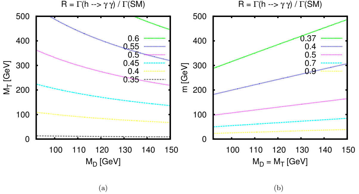
Figure 11: Contour lines for the ratio, R = \Gamma(h \rightarrow \gamma\gamma) / \Gamma(h \rightarrow \gamma\gamma)_{\text{SM}} , for the decay rate of Higgs boson decays into two photons over the SM prediction on (a) M_D vs. M_T plane with m = 200 GeV and (b) on M_D vs. m plane with M_T = M_D .
