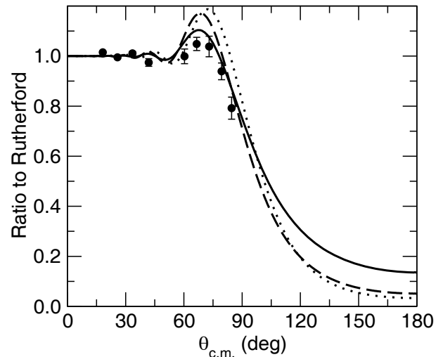
Fig. 1. Calculated quasi-elastic scattering angular distributions for 18.5 MeV ^8\text{Li} + ^{90}\text{Zr} compared with the data. The dotted, dashed and solid curves denote the no-coupling, CC and CRC calculations, respectively, see text for details. Note the linear cross section scale.
