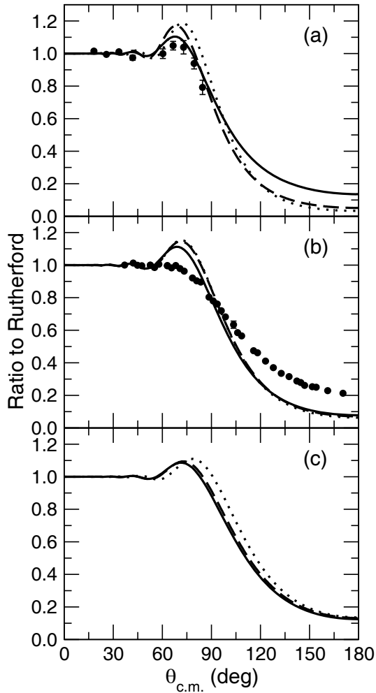
Fig. 2. (a) Quasi-elastic scattering angular distributions for 18.5 MeV {}^8\text{Li} + {}^{90}\text{Zr} , as in fig. 1. (b) Elastic scattering angular distributions for 18.9 MeV {}^6\text{Li} + {}^{90}\text{Zr} . Filled circles denote the data of ref. [41]. (c) Quasi-elastic scattering angular distributions for 18.5 MeV {}^7\text{Li} + {}^{90}\text{Zr} . Dotted, dashed and solid curves denote no-coupling, CC and CRC calculations, respectively, see text for details.
