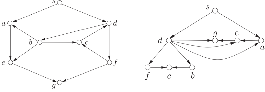
Figure 1.3: A flow graph and its corresponding derived graph.
