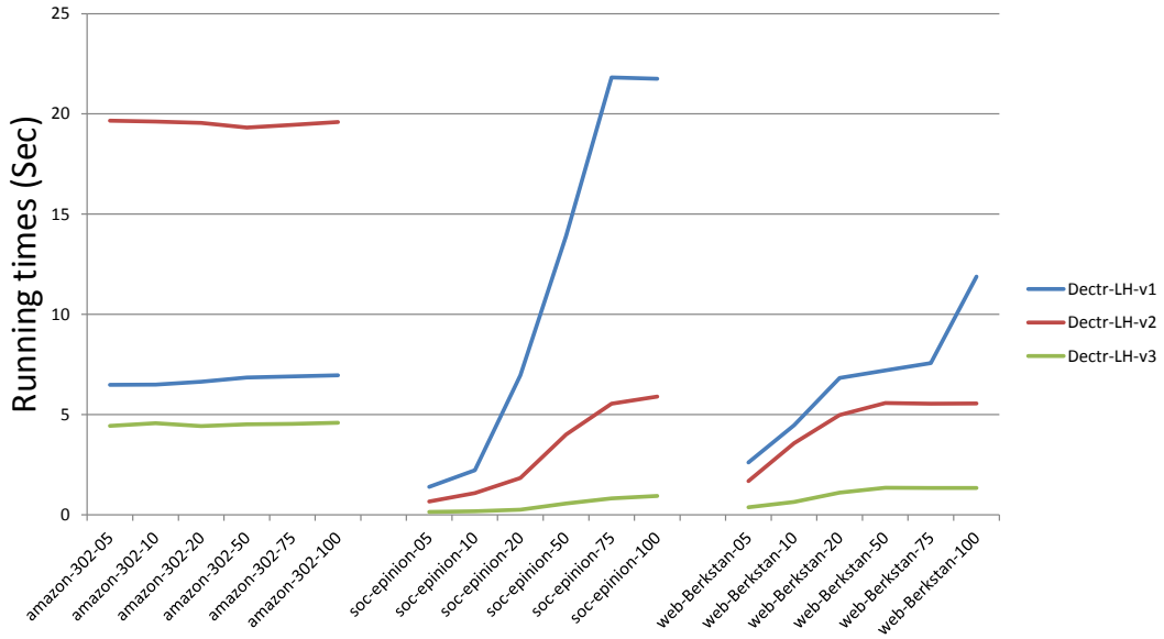
Figure 4.1: Average running times (in seconds) of three versions of Decr-LH that handle the deletion of a bridge (x, y) as described in Section 3.2. Decr-LH-v1 applies method (a) (running a static algorithm from scratch), Decr-LH-v2 applies method (b) (handling each edge (u, v) with u \in D(y) and v \in D \setminus D(y) as a regular deletion), while Decr-LH-v3 applies the improved method of Section 3.2.
