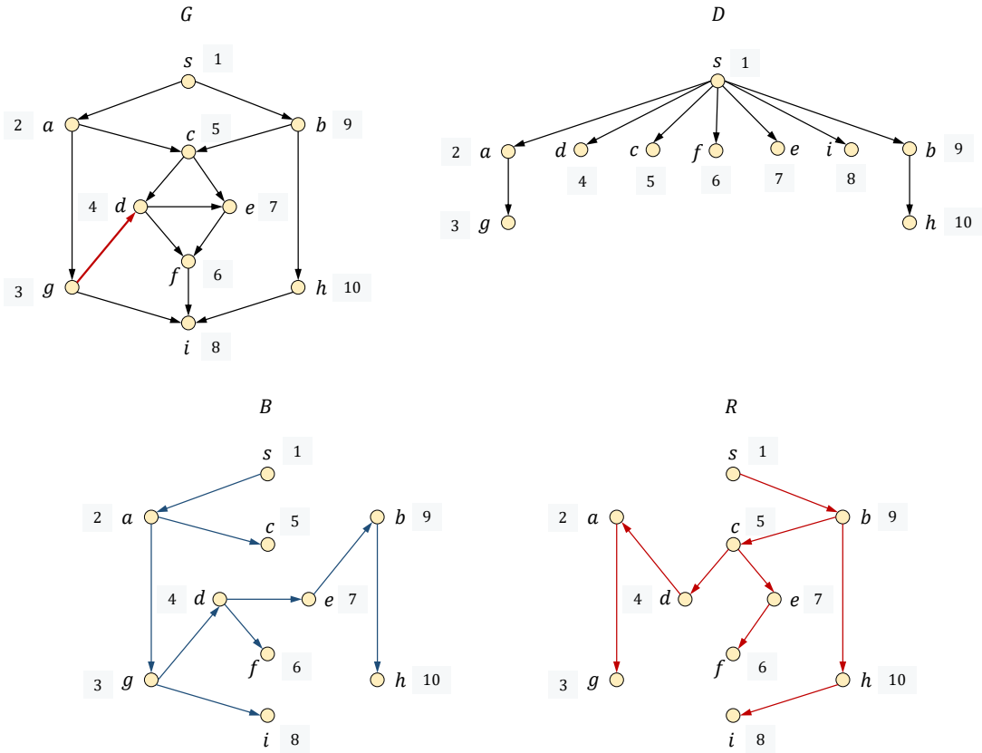
Figure 1.2: The flow graph of Figure 1.1 and two strongly divergent spanning trees B and R .
