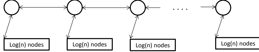
Figure 2.1: Representatives list data structure
