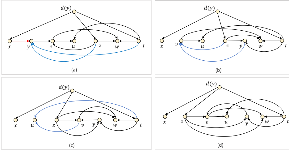
Figure 3.1: An example of propagation of changes in the low-high order after the deletion of an edge. Vertices are arranged from left to right in low-high order. (a) After the deletion of (x, y) , y violates the given low-high order. (b)-(c) Moving y between z and t causes a new violation at vertex v , which in turn causes another violation at vertex u after v is placed between z and y . (d) The low-high order is finally restored when we place u between v and t .
