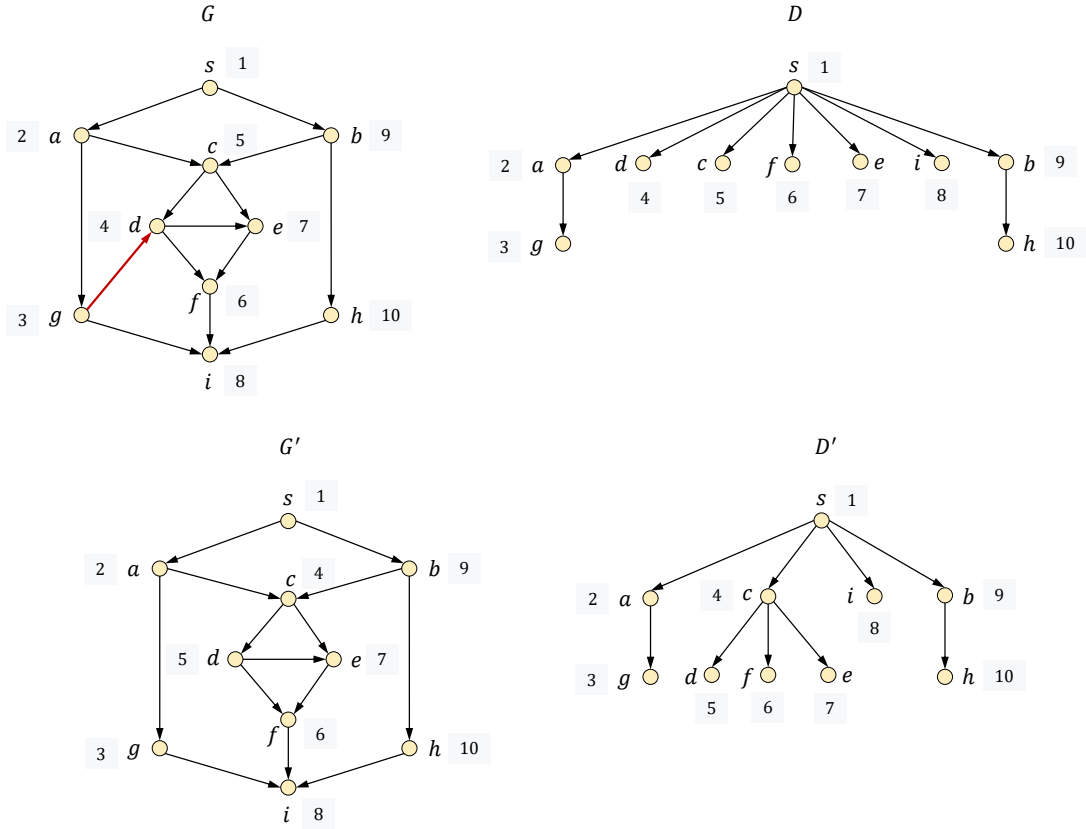
Figure 1.1: (Top) A flow graph G and its dominator tree D . The numbers correspond to a preorder numbering of D that is a low-high order of G . (Bottom) The flow graph G' and its dominator tree D' after the deletion of edge (g, d) .
