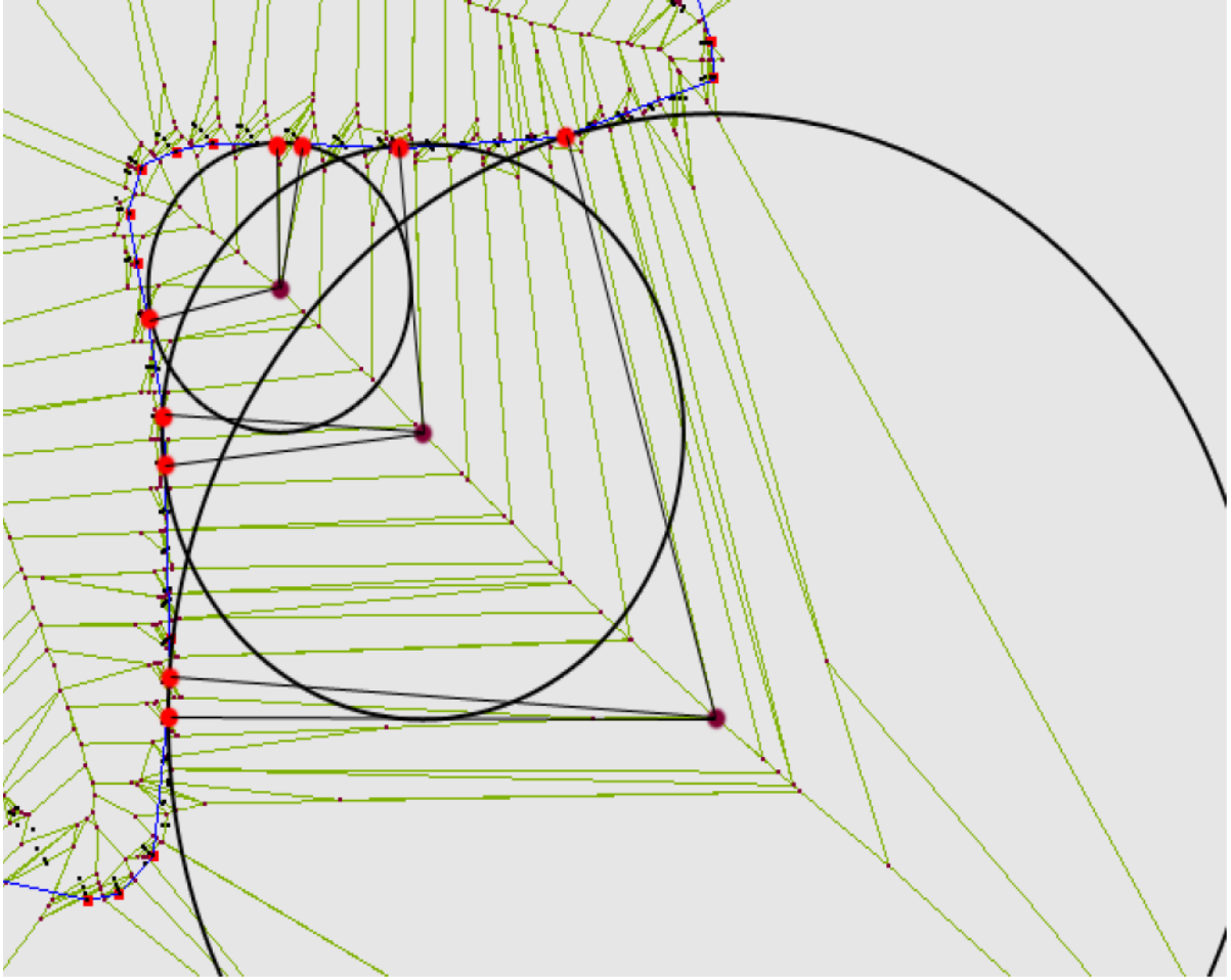
Figure 4.4: Detail of a cross section of the handle of the screwdriver point cloud. The largest empty circle of a Voronoi vertex is used to identify additional feature points and update the curve.
