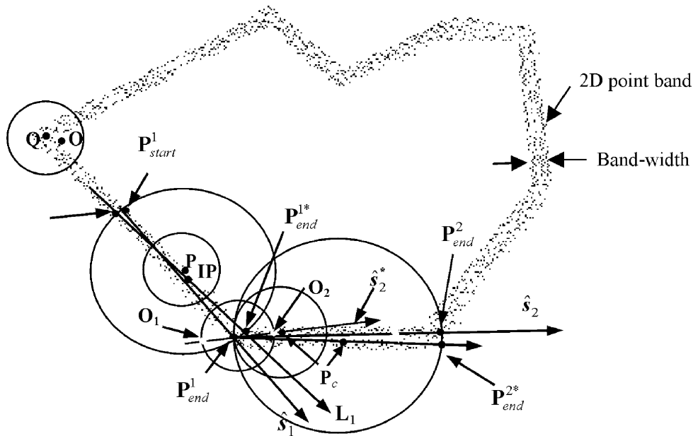
Figure A.3: Initial point IP determination and first, second segment construction.
