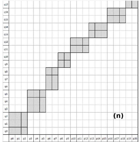
Figure 5.3: The recursive process of the contour triangulation (cont.).
