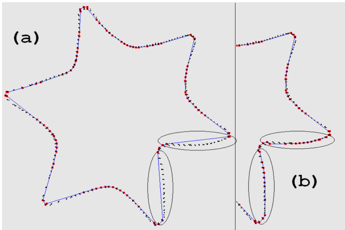
Figure A.6: A cross section of the handle of the screwdriver point cloud. (a) Second iteration of the Alternating Convex Hull Method. There are still some regions where the curve doesn't fit the points accurately. (b) Third iteration of the Alternating Convex Hull Method. The curve now describes the slice points more accurately.
