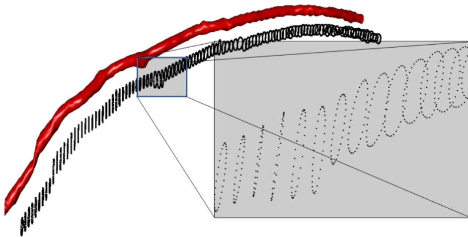
Figure 7.1: The model of an artery, and the points that came as input. Input: A 3D point set of an artery, organized in 2D slices of 80 points, provided from a CT Scan. Output: A collection of closed NURBS curves that interpolate the points of each slice accurately. These curves are used for reconstructing the surface of the model (red surface on the top left).
