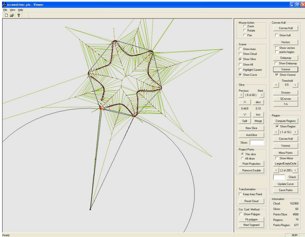
Figure A.8: A cross section of the handle of the screwdriver point cloud. The largest empty circle of the farthest Voronoi vertex is used to identify the next group of feature points.
