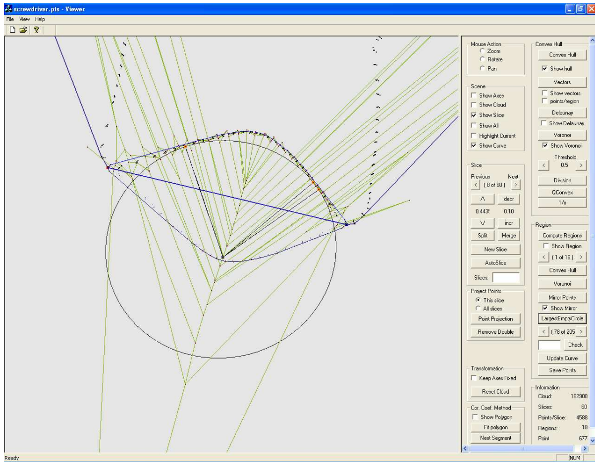
Figure A.9: A cross section of the handle of the screwdriver point cloud. By choosing a Voronoi vertex that is the farthest inside a bounded region we can identify feature points that are not too close to each other, and update the fitting poly-line faster.
