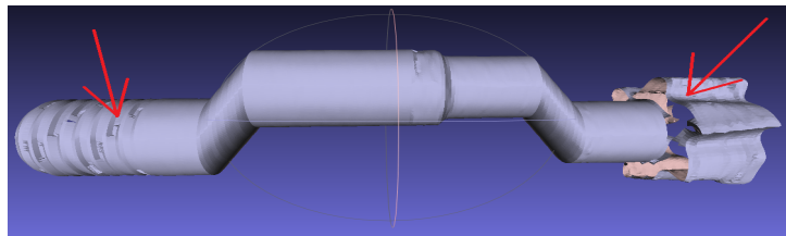
Figure 8.4: The surface of the drill bit model, reconstructed with the ball pivoting algorithm in MeshLab.
