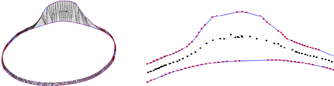
Figure 5.4: Cross sections in the area under the chin of the cycladean idol point cloud. (Left) A triangulation is computed between the contours of the two cross sections. The three vertices of each triangle correspond to a Voronoi region and define a circle (the largest empty circle), the center of which is identified as feature point for the new intermediate cross section. (Right) A detail from the area under the chin of the cycladean idol. The newly computed feature points are positioned in 3D space and have to be projected to the corresponding 2D plane between the two existing cross sections, to form the feature poly-line of the intermediate cross section.
