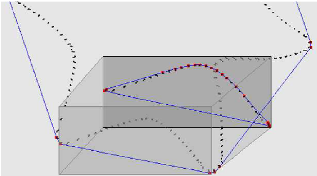
Figure A.5: Detail of a cross section of the handle of the screwdriver point cloud. The points in the highlighted region are isolated and the convex hull of these points is computed to identify the next set of feature points for the curve.
