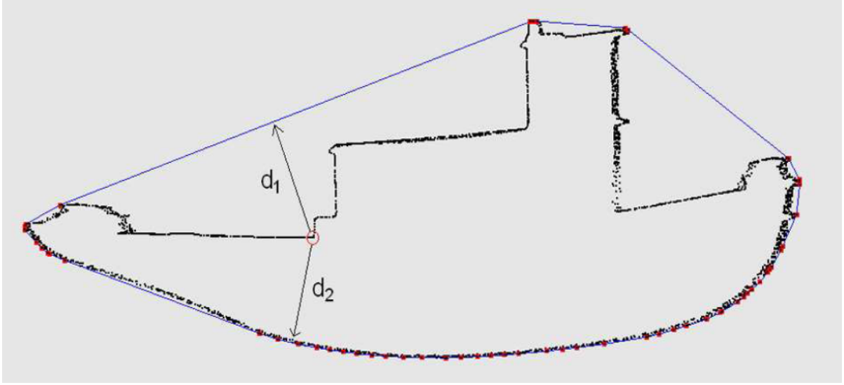
Figure 4.3: A cross section of the point cloud of the Cyberware boat [1]. The points in the highlighted area (small circle) are located closer to a region other than they should be assigned to ( d_2 < d_1 ). We need to use the information of their neighboring points to assign them to the correct region.
