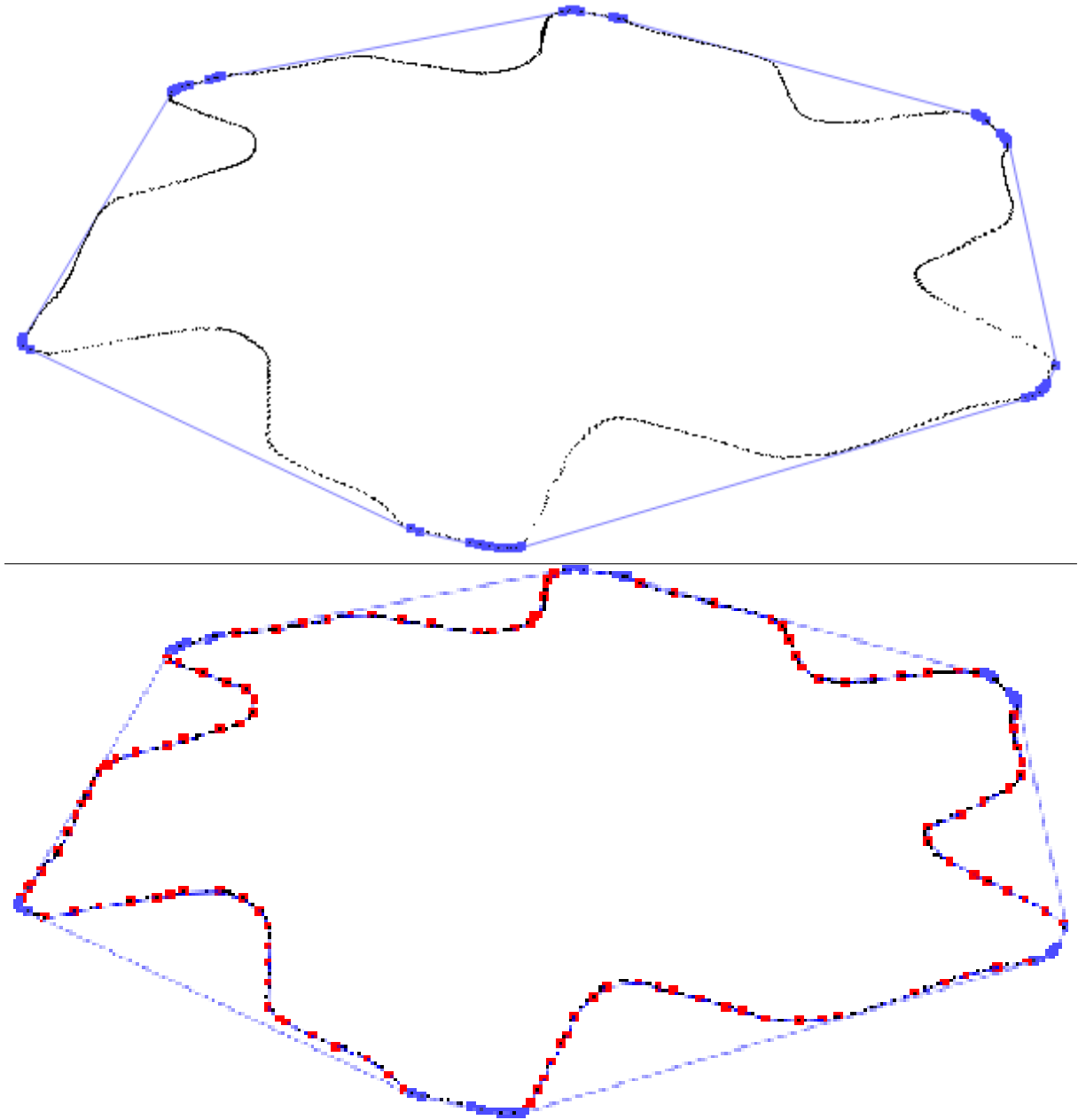
Figure 4.9: A cross section of the twist drill bit point cloud. The points of a cross section are processed as an individual 2D point set. (Top) The convex hull of the point set (blue points) provides the initial feature poly-line. (Bottom) The feature poly-line is updated as new feature points are added in regions where the point set is not accurately described (red points).
