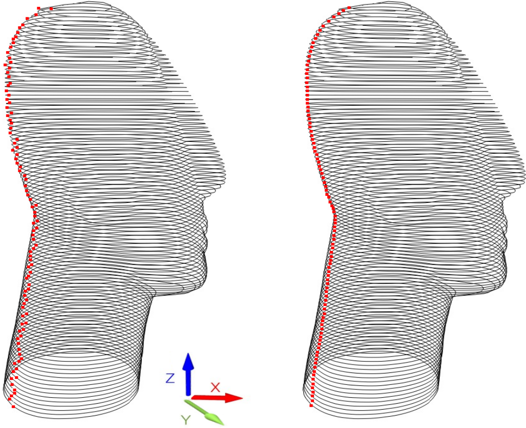
Figure 5.9: (Left) The start/end point p_i on each cross section is set to the feature point with p_x = \min(x) and p_y = \min(|y|) . The points are not aligned and the surface reconstruction will suffer from irregularities. (Right) By re-sampling the curves we are able to set the start/end points p_i to the points with p_x = \min(x) and p_y = 0 . The points are now aligned and the surface reconstruction becomes robust.
