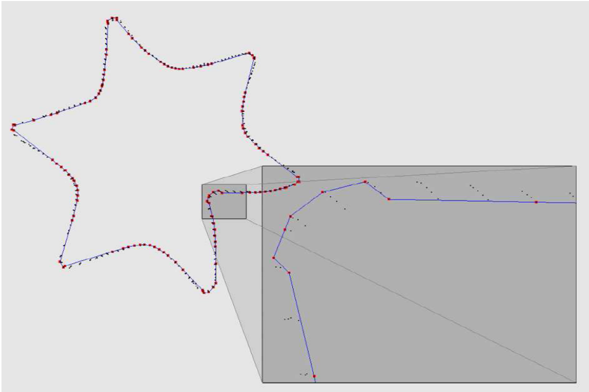
Figure A.7: A detail of a cross section of the handle of the screwdriver point cloud. The convex hull method identifies internal and external slice points alternatively as feature points. If this affects the curve significantly, the feature poly-line will have irregularities when switching between regions.
