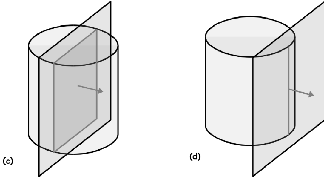
Figure 3.3: The slicing direction is an essential parameter for the modeling process. (c) The slicing direction is vertical to the cylinder axis. The points of a cross section form a rectangle. (d) The slicing direction is vertical to the cylinder axis. The points of the last cross section form a line.
