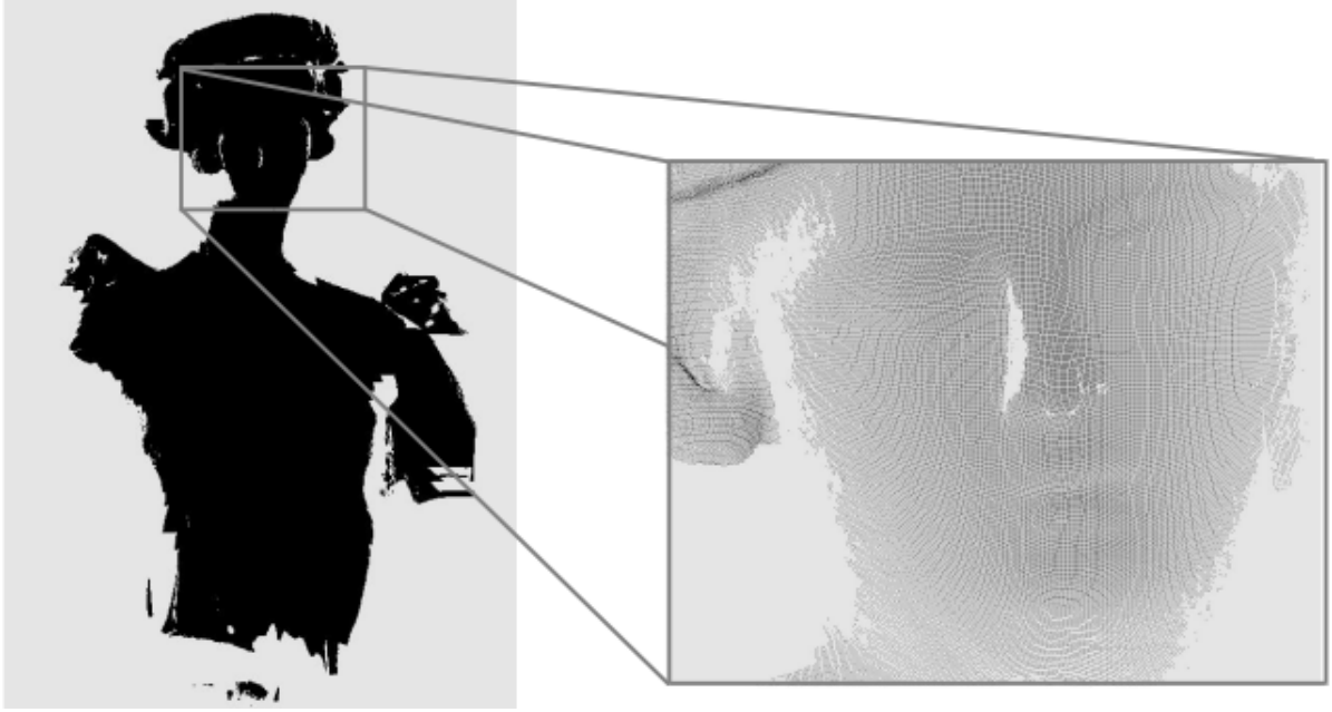
Figure 3.1: The point cloud of a female figure. The only information provided are the [x, y, z] coordinates of points on the surface of the model.
