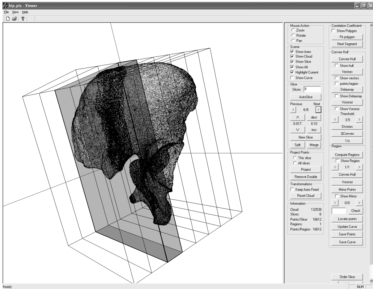
Figure 3.8: The Cyberware hip bone. The proper slicing direction is not obvious in this model, as the medial axis of the cloud is not a simple curve.
