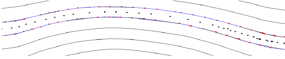
Figure 5.1: In case a new intermediate cross section is required, it is constructed from the Voronoi centers of the points of two adjacent feature poly-lines.
