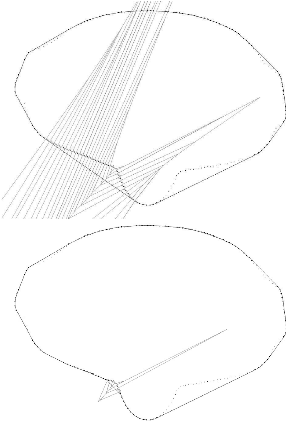
Figure 4.7: A cross section of the cycladean idol point cloud. For the feature polyline to fully describe a region, several iterations may be required. (Top) The first iteration of our method applied on a region. (Bottom) The second iteration for the small region.
