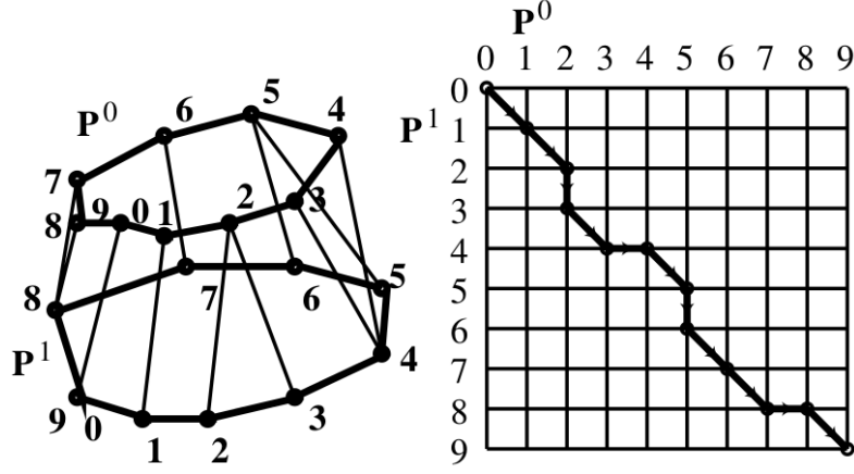
Figure 5.2: For the contour triangulation, the connectivity of the points is expressed as a monotonically decreasing path in a tabular scheme that specifies which points participate in each triangle or quad.
