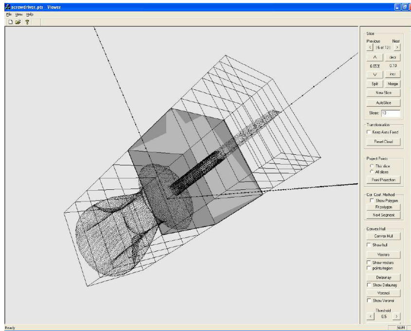
Figure 3.5: The Cyberware Screwdriver. The point cloud may be sliced into cross sections of variable thickness. The principal axis of the point cloud usually matches the ideal direction for slicing the cloud.
