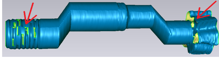
Figure 8.3: The drill bit model edited with Geomagic Studio. Some triangles at the screw threads and the drill seem to have been incorrectly computed.
