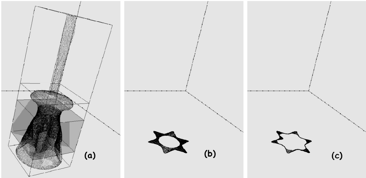
Figure 3.6: Instances of the sliced screwdriver with different values of thickness. When the highlighted cross section from (a) is projected on its 2D plane, we get the slice in (b). Having cross sections with half its thickness will project to slice (c).
