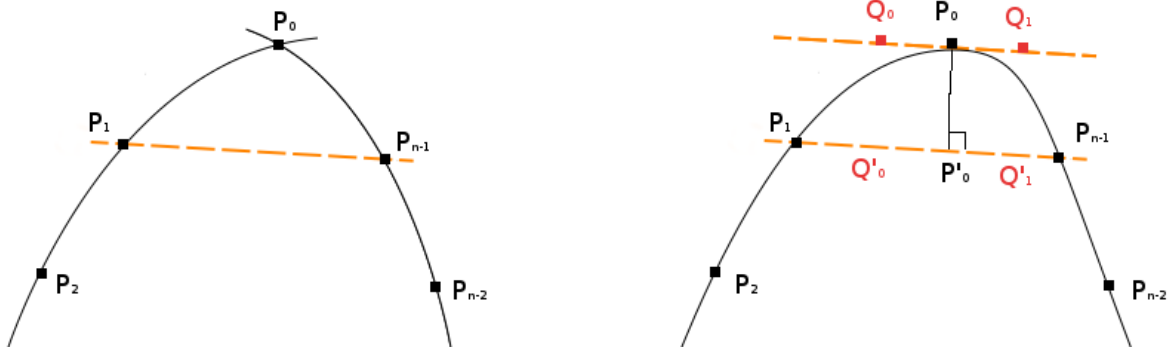
Figure 5.5: To ensure G^1 continuity on the end points we insert two more points that enforce collinearity of the three points near the start/end point of the curve.
