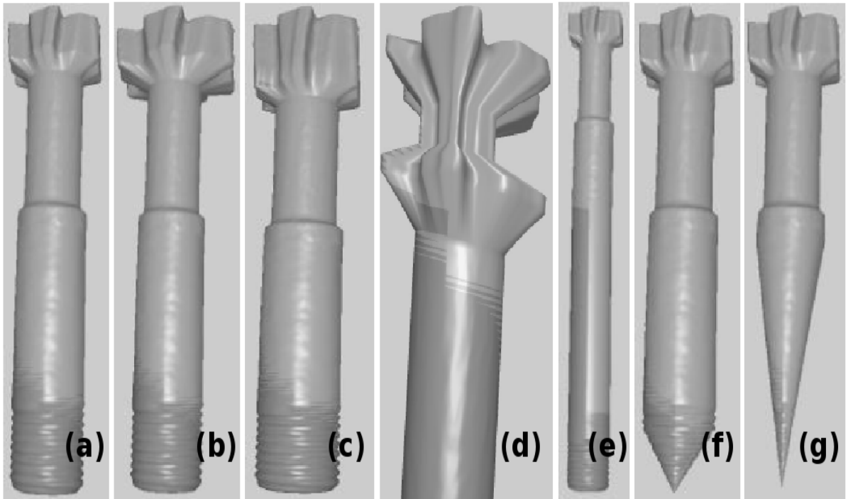
Figure 6.5: Transformations applied on the twist drill bit point cloud.
