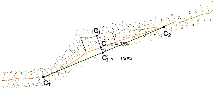
Figure 7.6: The centroid C_i is getting closer to the line segment [C_1, C_2] , as the parameter \alpha increases. For \alpha = 0 we have C'_i = C_i , and for \alpha = 100\% the centroid C_i is projected on the line segment [C_1, C_2] .
