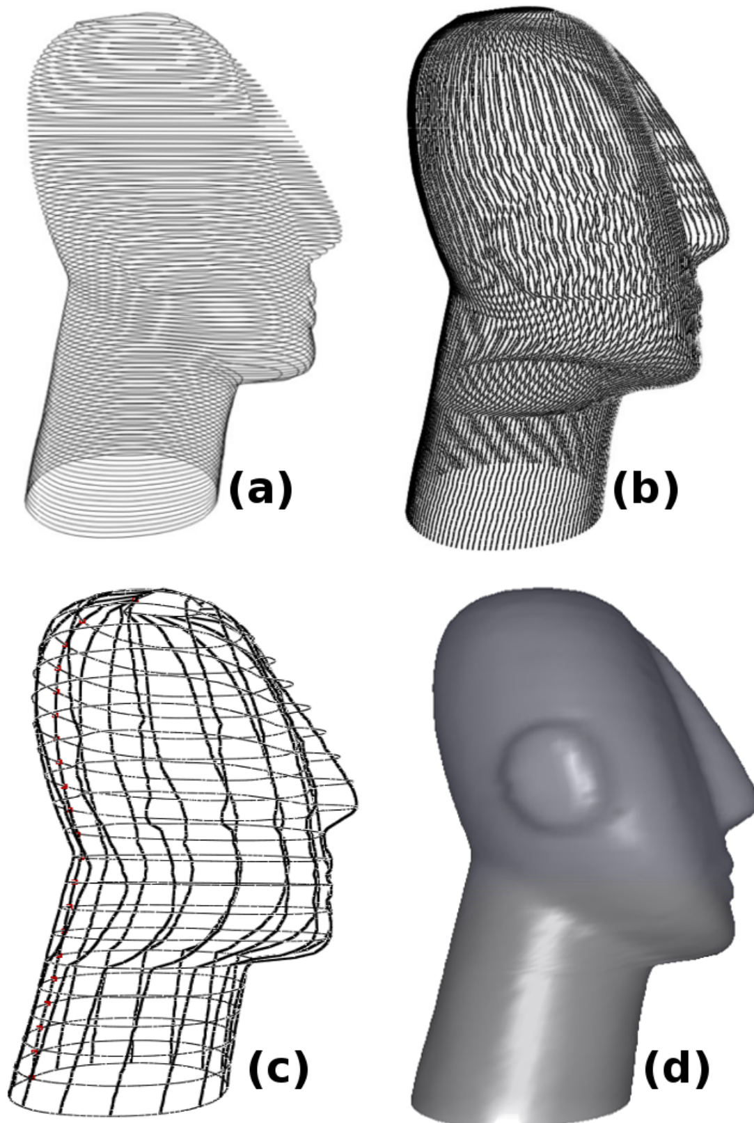
Figure 5.11: The resulting model: (a) the B-Spline curves of the cross sections, (b) the vertical curves, (c) a thinned visualization of the cross sections combined with the vertical curves, and (d) the reconstructed surface.
