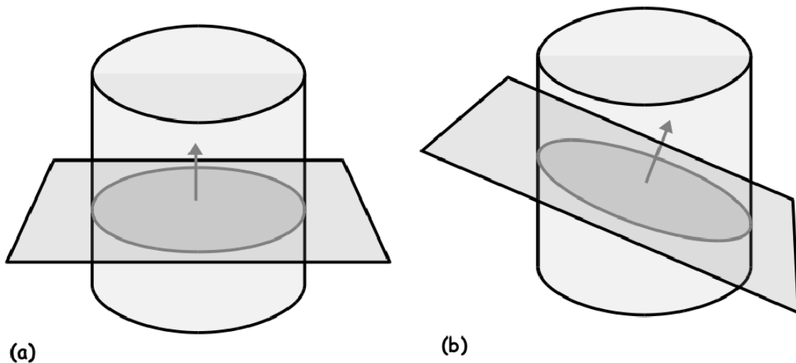
Figure 3.3: The slicing direction is an essential parameter for the modeling process. (a) The slicing direction matches the cylinder axis. The points of a cross section form a circle. (b) The slicing direction is different than the cylinder axis. The points of a cross section form an ellipse.
