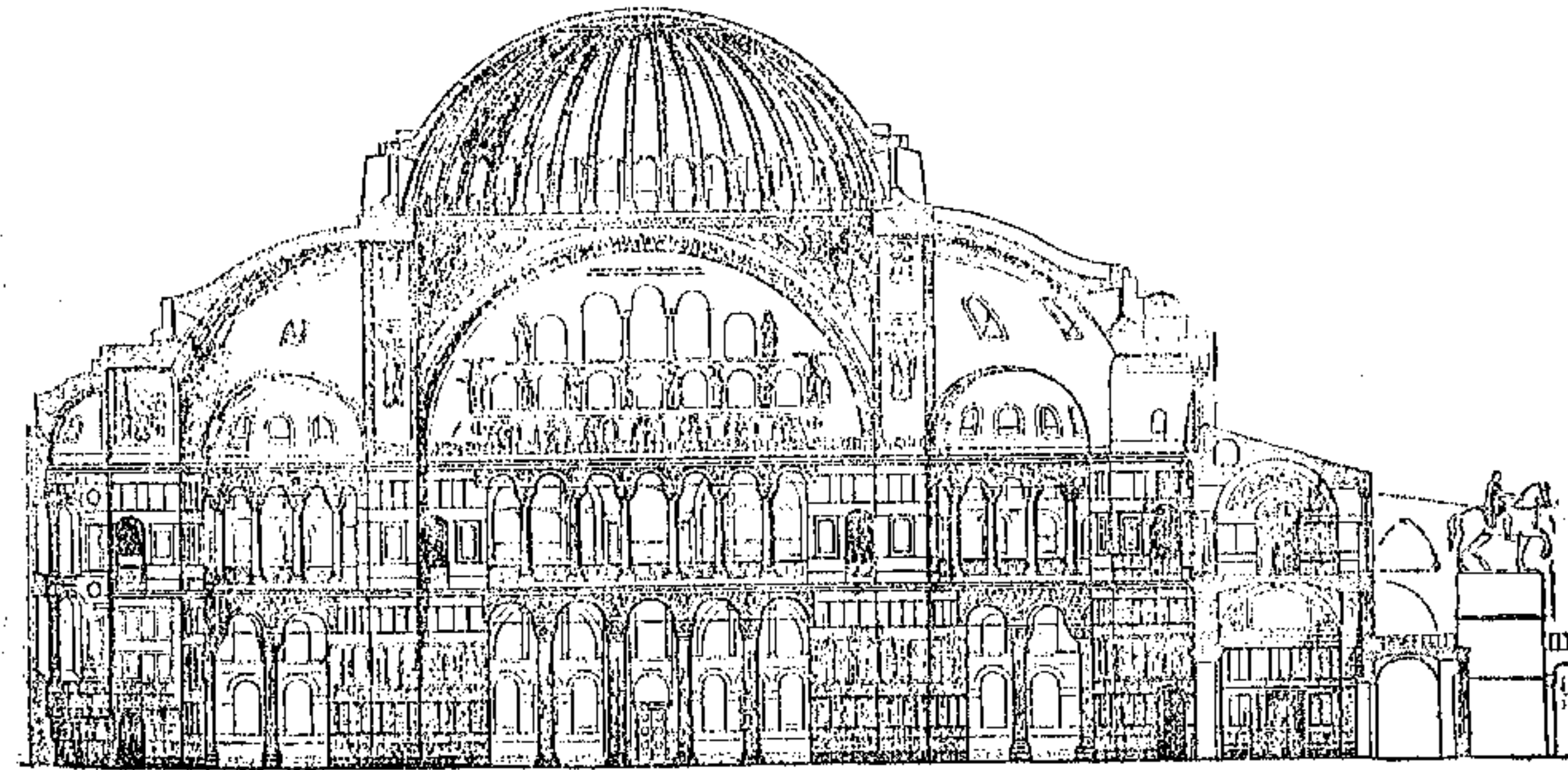
Κατὰ μῆκος τομὴ τοῦ ἐν Κωνσταντινουπόλει ναοῦ τῆς τοῦ Θεοῦ Σοφίας.
