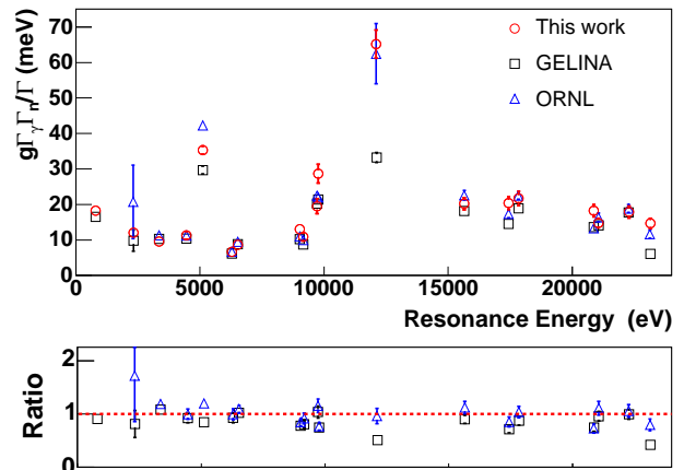
FIG. 5: (Color online) Comparison of the radiative capture kernels derived from the measurements at n_TOF, GELINA and ORNL. The capture area shown at 2.3 keV for ORNL corresponds to an estimation reported in Ref. [6]. The capture area shown at \sim 12 keV, corresponds to the sum of the three resonances in that region.
