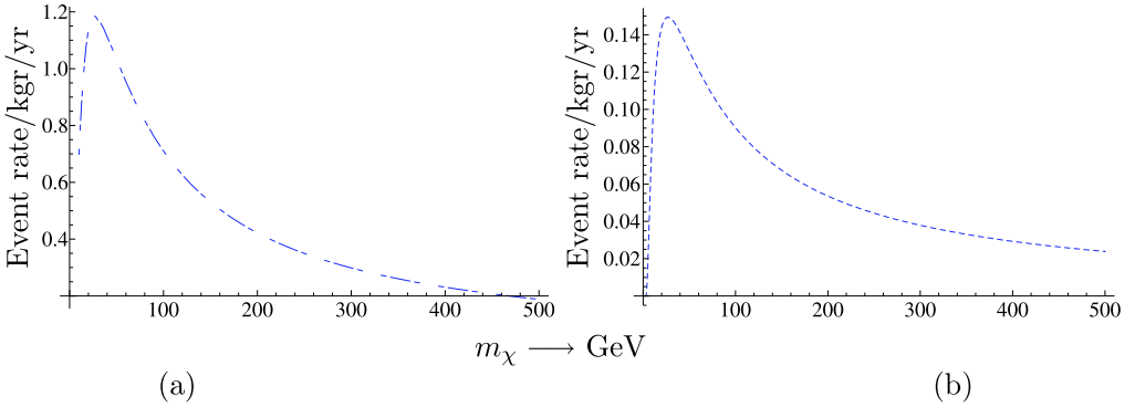
Fig. 4. The same as in Fig. 3 in the case of the light target ^{19}\text{F} .
