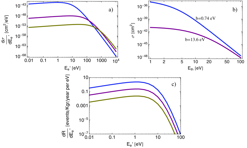
Fig. 6. (a) Predictions for d\sigma/dE'_e as a function of the ejected electron energy E'_e . The target is assumed to be a hydrogenic atom in the ground state with Z = 1, 3, 6 (from top to bottom). (b) The total cross section for process (4.43) as a function of the experimental threshold energy for two binding energies. (c) The differential event rate as a function of the electron energy and various WIMP masses (10, 100, 1000) GeV from (top to bottom). Other parameters not shown, are taken from Eq. (4.65).
