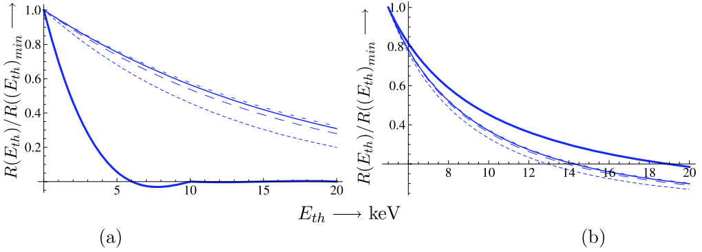
Fig. 5. The quantity R(E_{th})/R((E_{th})_{min}) , i.e., the ratio of the event rate at a given threshold divided by that at the lowest threshold considered, as a function of the threshold energy. In (a) as predicted by traditional mechanisms (lowest threshold assumed zero). In (b) as predicted by the present model (now due to the need for a cut off the lowest threshold energy employed was 5 keV). The thick line, short dash, long dash, fine line and long short dash correspond to WIMP masses 10, 50, 100, 200 and 500 GeV, respectively.
