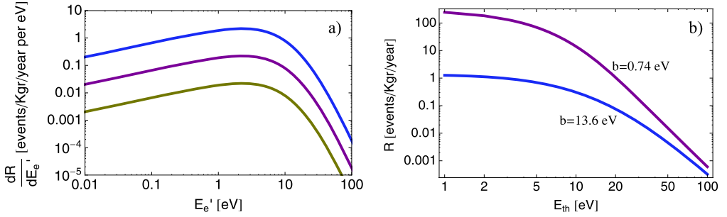
Fig. 8. (a) Differential event rate of Dirac WIMP scattered off hydrogen ( Z = 1 , A = 1 ) target electrons per year per kg as a function of ejected electron energy E_e' in eV. Three different WIMP masses have been assumed: m_\chi = 10, 100, 1000 GeV, from top to bottom, respectively. (b) The total event rate as a function of the experimental threshold energy for m_\chi = 100 GeV for two different binding energies. Other input parameters are taken from Eq. (4.67) for the massive mediator.
