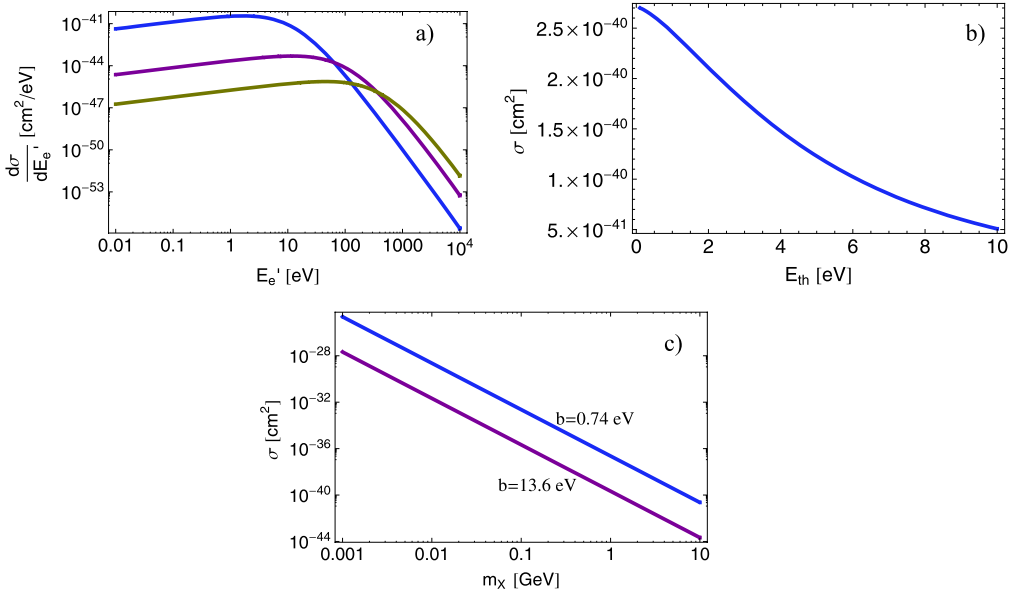
Fig. 7. (a) Predictions for d\sigma/dE'_e as a function of the ejected electron energy E'_e . The target is assumed hydrogenic atom with Z = 1, 3, 6 (from top to bottom) in the ground state. (b) The total cross section as a function of threshold energy. (c) The total cross section as a function of m_\chi for two different binding energies. We assume a Dirac WIMP, E_{\text{th}} = 0 eV and input parameters from Eq. (4.67) if not stated otherwise.
