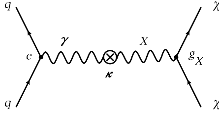
Fig. 2. A Feynman diagram leading to the direct interaction of the WIMP \chi to the quarks relevant for direct detection of dark matter. The process is mediated by the physical photon. The cross indicates merely that the exotic gauge boson has a small admixture of the photon. Similarly the WIMP can also couple to electrons.
