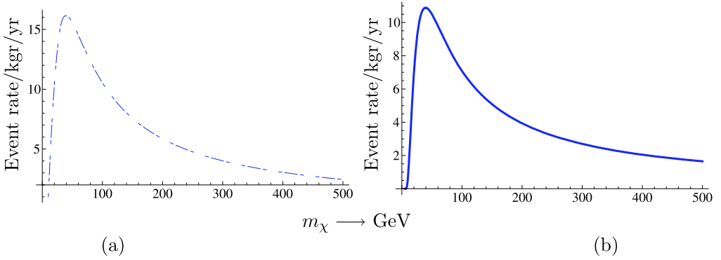
Fig. 3. The total rates for traditional WIMP searches assuming a nucleon cross section \sigma_N = 10^{-43} \text{ cm}^2 in (a). The case of the photon mediated process considered in this work is exhibited in (b). Both refer to the case of a heavy target ( A = 131 ) and were computed assuming an energy threshold of 5 KeV. The results for the iodine target used by the DAMA experiment are almost identical.
