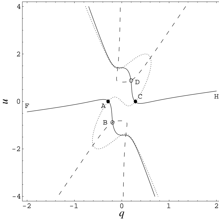
Figure 2: A solution interpolating between the Randall–Sundrum solution at z = +\infty and a naked singularity (see (59) for the case \rho_2 ) at z = 0 . There are two (physically equivalent) branches CH and AF . There are other solutions that encounter ( D or B ) non-resolvable singularities in the derivatives dq/dy, du/dy (dashed curves). The dotted curve (for u \neq 0 ) corresponds to the exact solutions of eq. (53).
