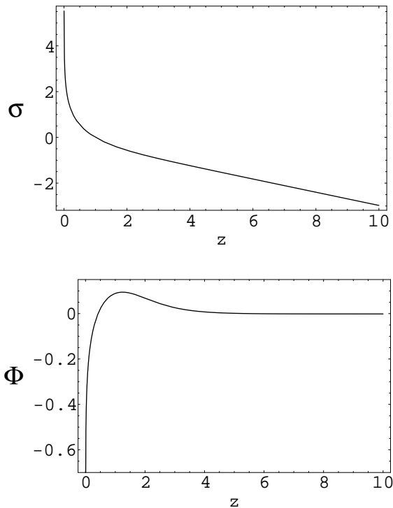
Figure 3: The metric \sigma(z) and dilaton \Phi(z) as functions of z interpolating between a RS type solution ( q_0 = -\sqrt{1/12} ) at z = +\infty and a naked singularity (see (59) for \rho_2 ) at z = 0 . The existence of this solution implies the dynamical restriction of the bulk space-time to the positive z axis.
