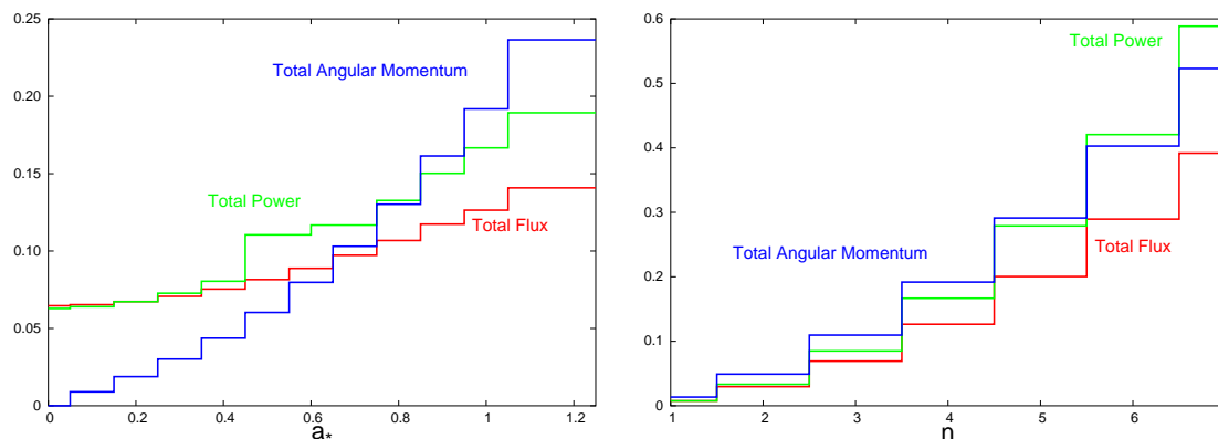
Figure 12: Total emissivities for scalar emission on the brane from a rotating black hole as a function of (a) a_* , for n = 4 , and (b) n for a_* = 1 .
