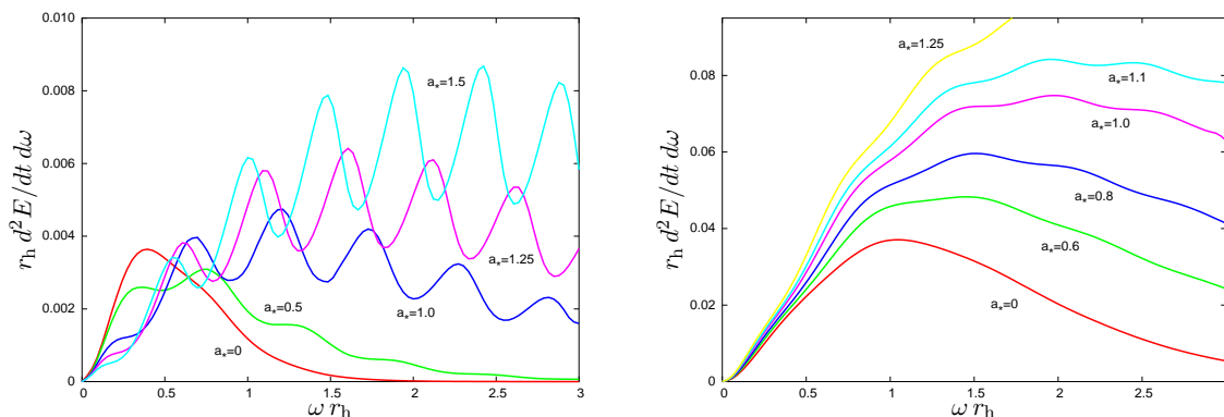
Figure 6: Power emission spectra for scalar particles on the brane from a rotating black hole, for (a) n = 1 , and (b) n = 4 , and various values of a_* .
