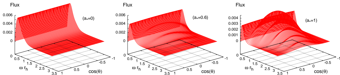
Figure 4: Angular distribution of the flux spectra for scalar emission on the brane from a rotating black hole, for n = 1 and a_* = (0, 0.6, 1) .
