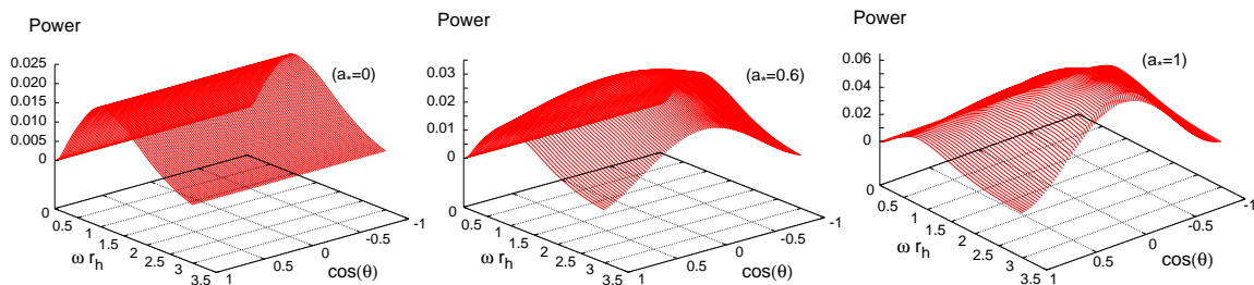
Figure 9: Angular distribution of the power spectra for scalar emission from rotating black holes, for n = 4 and a_* = (0, 0.6, 1) .
