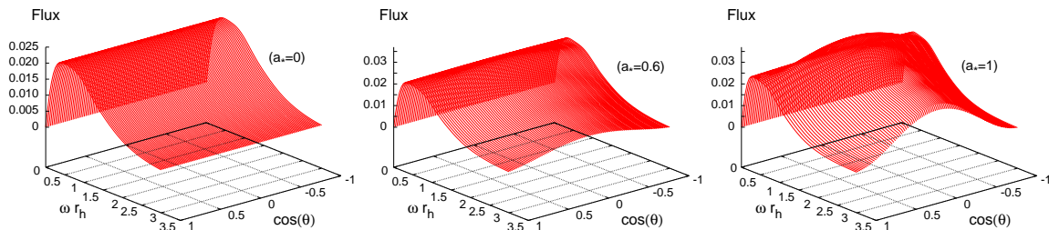
Figure 5: Angular distribution of the flux spectra for scalar emission on the brane from a rotating black hole, for n = 4 and a_* = (0, 0.6, 1) .
