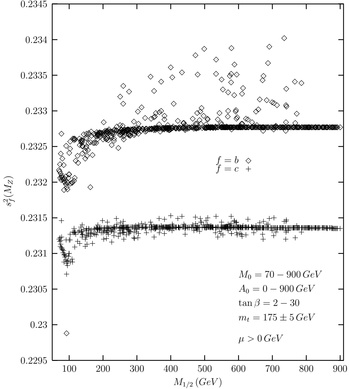
Figure 4 : The effective weak mixing angles s_c^2 and s_b^2 . In the region M_{1/2} \rightarrow 900 \text{ GeV} , the two angles are separated from each other. The dispersion of points around the central value for M_{1/2} > 200 \text{ GeV} is due to the variation of the top mass. For the limiting behaviour to be more clearly exhibited, in this figure and in figures 3,7 and 8 we do not display the dispersion of points for M_{1/2} > 800 \text{ GeV} .
