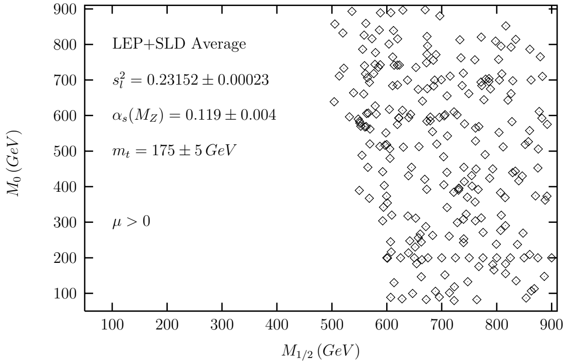
Figure 9 : Acceptable values in the M_{1/2} - M_0 plane according to the LEP+SLD data. The values of \tan \beta and A_0 are taken in the region 2 – 30 and 0 – 900 GeV, respectively. Only large values of M_{1/2} are acceptable.
