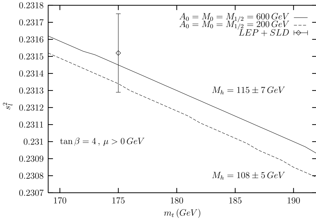
Figure 5 : MSSM predictions for s_l^2 as a function of m_t for two different characteristic values of the soft breaking parameters. The corresponding values of the light Higgs mass and their errors due to the variation of m_t are indicated.
