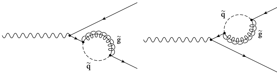
Figure 2c : Supersymmetric QCD corrections to the Zq\bar{q} vertex from gluino and squark contributions.
