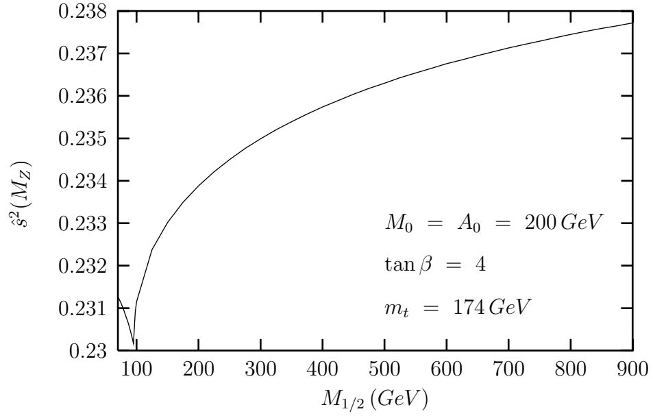
Figure 1: The values of the running weak mixing angle \hat{s}^2 at M_Z in the \overline{DR} scheme defined as a ratio of gauge couplings for various input universal soft gaugino masses M_{1/2} for particular input of M_0 , A , \tan\beta and m_t . The strong dependence of \hat{s}^2 on M_{1/2} near M_Z is due to the presence of sparticle thresholds.
