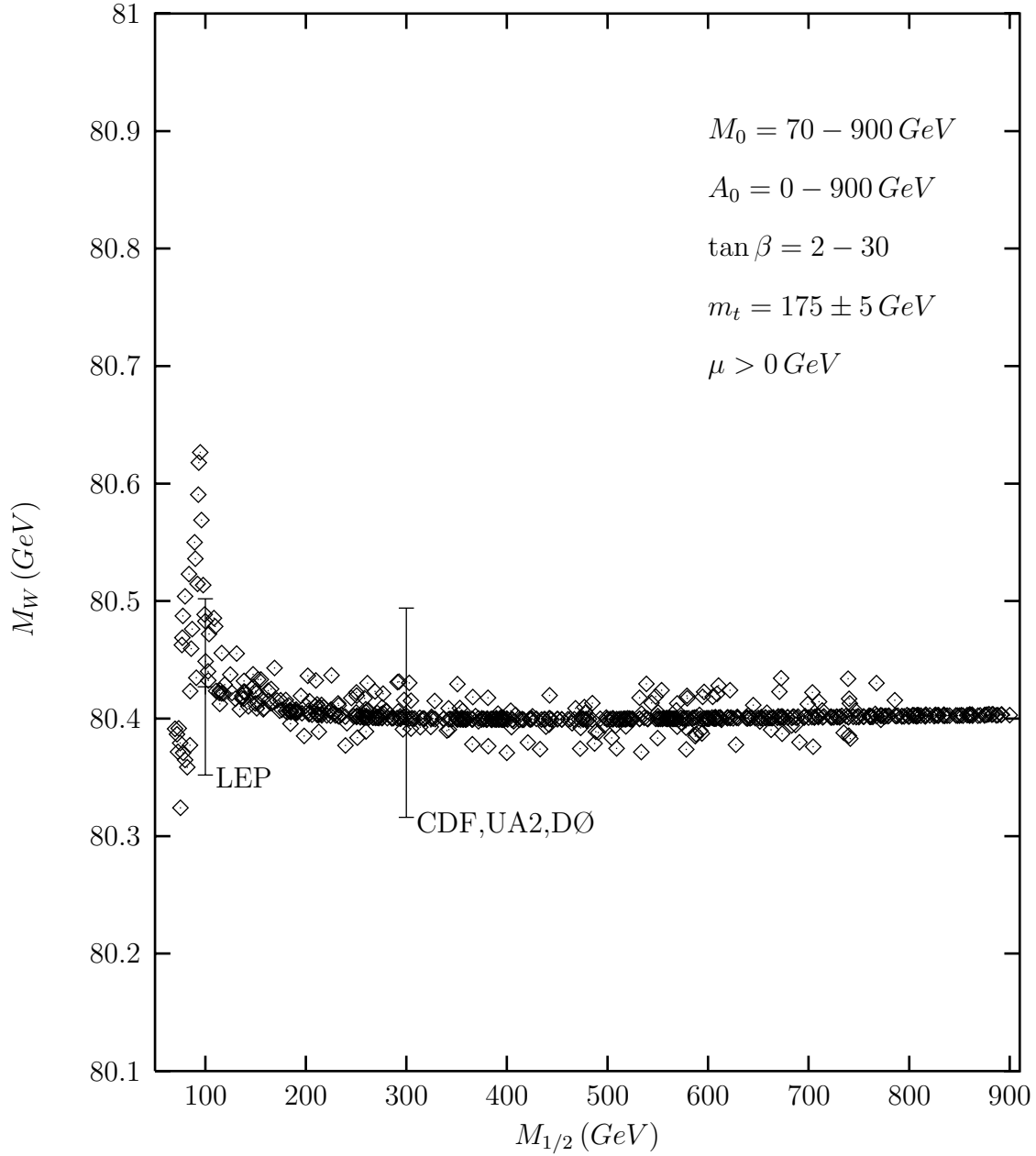
Figure 7 : MSSM prediction for the mass of the W-gauge boson as a function of the independent soft parameters M_{1/2} , M_0 and A_0 . The experimental value M_W = 80.427 \pm 0.075 ( M_W = 80.405 \pm 0.089 ) GeV obtained at LEP (CDF,UA2,DØ) is shown for comparison.
