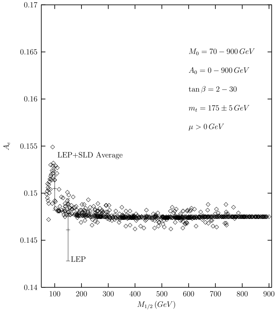
Figure 8 : The left-right asymmetry A_e in the MSSM as a function of M_{1/2} when we vary M_0 , A_0 , \tan \beta and m_t .
