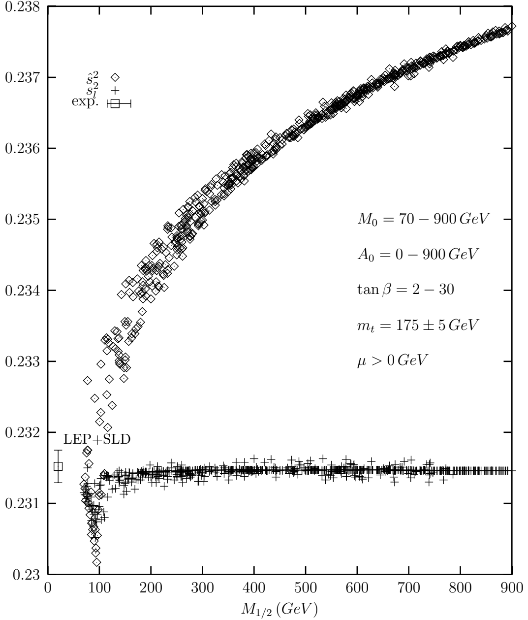
Figure 3 : The effective weak mixing angle s_l^2(M_Z) in comparison to the weak mixing angle \hat{s}^2(M_Z) versus M_{1/2} when the soft parameters M_0 , A_0 vary in the indicated regions. The width of each branch is due mainly to the variation on M_0 , for low M_{1/2} < 200 GeV, and to the variation of the top mass for M_{1/2} > 200 GeV. The effect of the variation of A_0 = 0 - 900 GeV and of \tan \beta = 5 - 28 on s_l^2 is negligible. The error bar show the measured value of s_l^2 = 0.23152 \pm 0.00023 , obtained at LEP and SLD. The MSSM value is in agreement with the LEP+SLD data for the bulk of the values in the soft parameter space.
