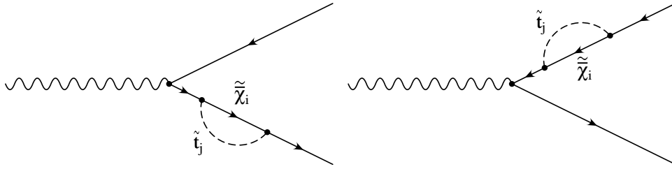
Figure 2a : Self energy chargino and squark corrections to the Zb\bar{b} vertex.
