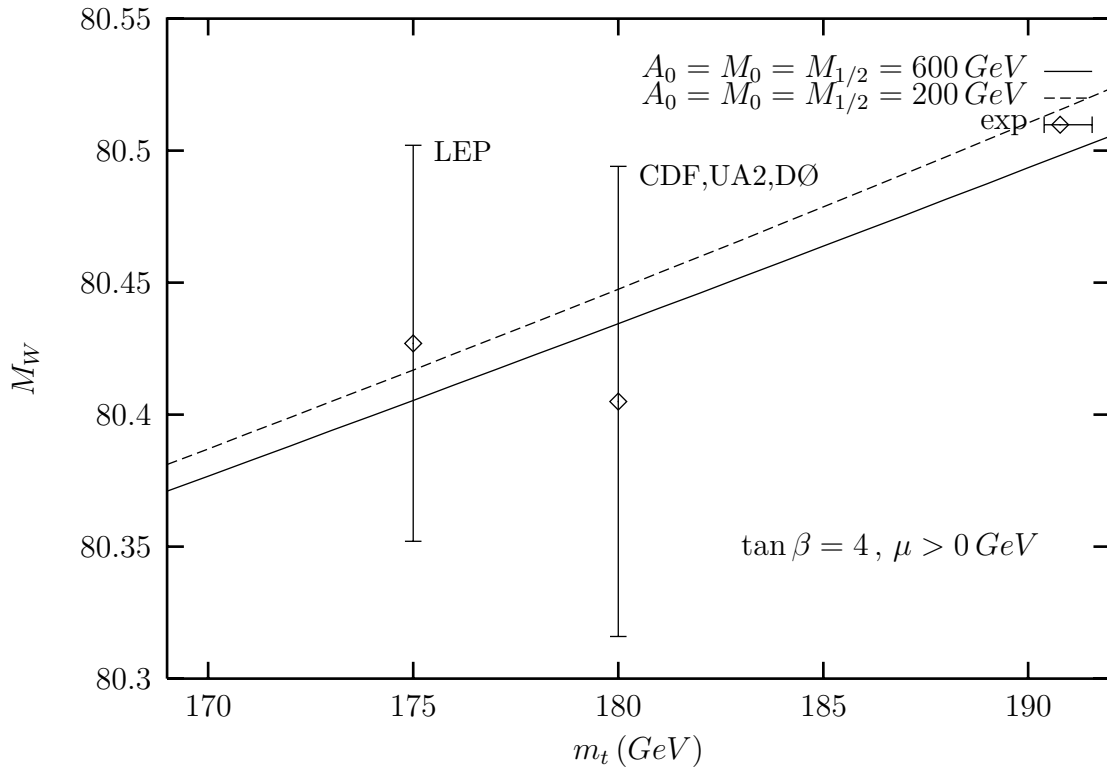
Figure 6 : MSSM predictions for physical mass of the W-boson as a function of m_t for the same inputs as in Figure 5.
