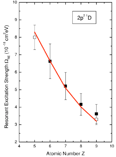
FIG. 9. (Color online) Resonance excitation collision strengths \Omega_{RE} plotted as a function of atomic number Z for the 2p^2 1D resonance taken in collisions of H-like ions with H_2 targets. Open squares: present measurements; solid squares: values extracted from the older data of Toth et al. [58] taken with a two-stage slit spectrometer; line: Hartree-Fock calculation. Good agreement is seen for the common point of fluorine at Z=9 .
