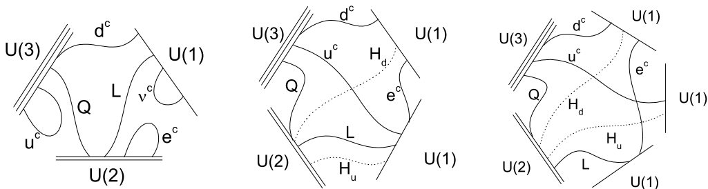
Figure 1: Selected Standard Model configurations with one, two and three abelian branes P = 1, 2, 3 .
