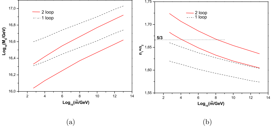
Figure 2: The M_S scale, (a), and the sum n_1 + n_2 , (b), as a function of \log_{10} \tilde{m} for the case where \alpha_3 = \alpha_2 at M_S . The bands correspond to the strong coupling experimental error at M_Z . The solid lines correspond to 2-loop running while the dotted ones to 1-loop.
