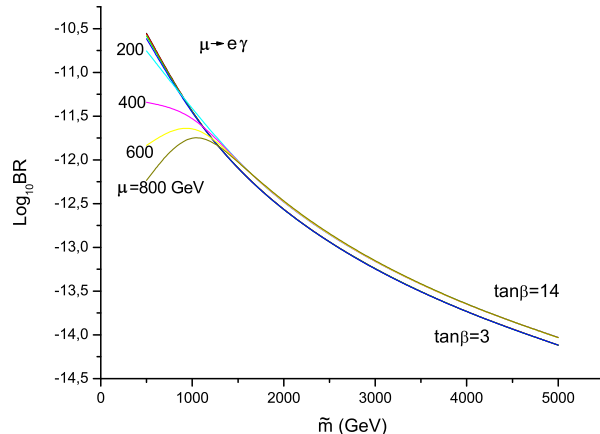
Figure 7: The (logarithm of the) branching ratio of \mu \rightarrow e\gamma as a function of \tilde{m} for \tan\beta = 3 and 14 and for \mu = 200, 400, 600, 800 GeV.
