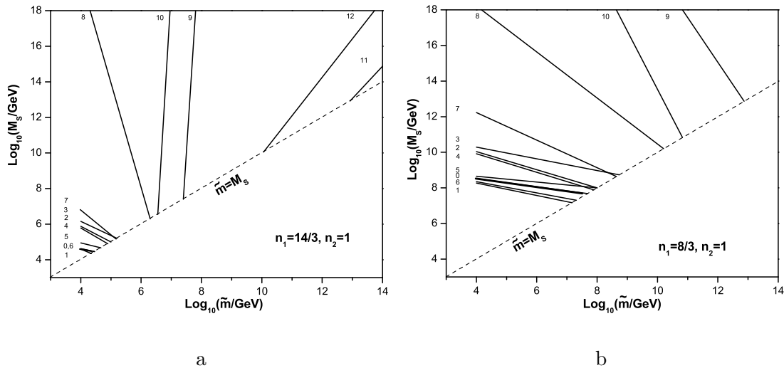
Figure 6: Plots of M_S vs \tilde{m} for the twelve models appearing in Table 4 and the two cases of the pair (n_1, n_2) . The thicker line corresponds to the case with no mirrors (0 model) while the label corresponds to the model as in Table 4.
