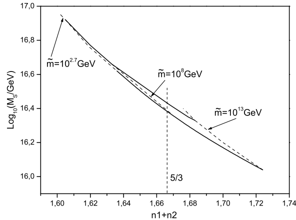
Figure 3: The M_S scale as a function of n_1 + n_2 . The two curves correspond to the a_3(M_Z) experimental uncertainty. Curves of constant \tilde{m} are shown for the values 10^{2.7} , 10^8 and 10^{13} GeV.
