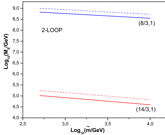
Figure 5: The M_S scale as a function of \tilde{m} , for 2-loop running for the models with (8/3,1) and (14/3,1) . Continuous lines correspond to the lower value of \alpha_3(M_Z) while dotted ones to the higher one.
