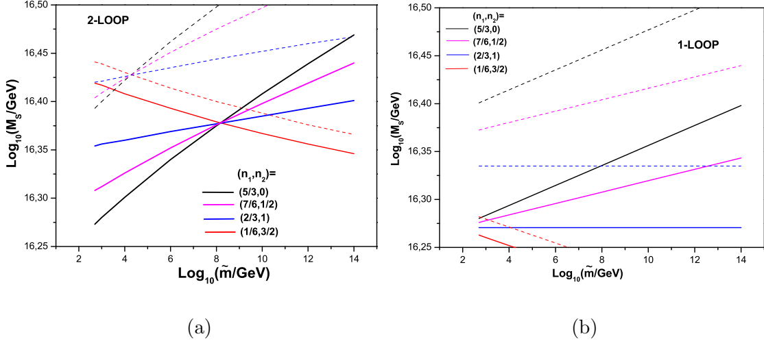
Figure 4: The M_S scale as a function of \tilde{m} , for 2-loop running (a) and 1-loop running (b), for the models having n_1 + n_2 = 5/3 . Continuous lines correspond to the lower value of \alpha_3(M_Z) while dotted ones to the higher one.
