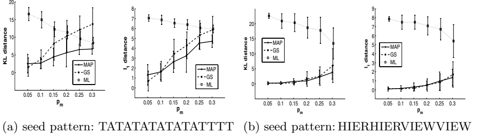
Fig. 1. Mean values and stds of KL and l_1 as calculated by the three methods in two single-pattern discovery problems (a), (b) using six values of noise parameter p_m .
