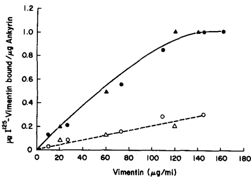
FIGURE 5 Binding of ^{125}\text{I} -vimentin to isolated ankyrin as detected by immunoprecipitation with a polyclonal anti-ankyrin antibody. \blacktriangle , \bullet , two separate assays with ^{125}\text{I} -vimentin, ankyrin, and anti-ankyrin (as specified in Materials and Methods) are shown. \Delta , controls (no ankyrin added); \circ , assay with normal rabbit serum instead of anti-ankyrin.
