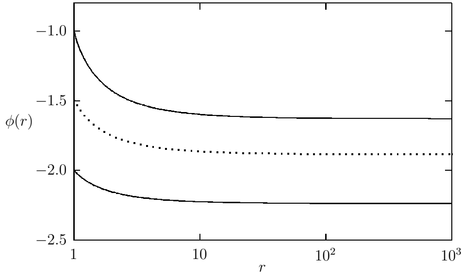
Figure 1: Dilaton field for r_h = 1 black hole. Each curve corresponds to a different solution characterized by a different initial value of \phi_h .
