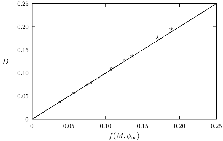
Figure 4: Dependence of the dilaton charge D on M and \phi_\infty for the r_h = 1 black hole. The function f(M, \phi_\infty) stands for the coefficient of 1/r in the eq.(65).
