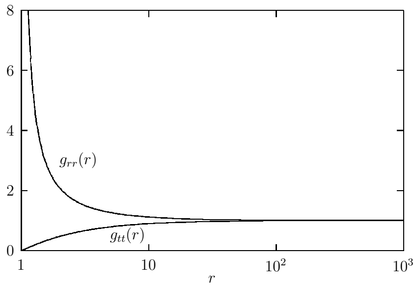
Figure 2: Metric components g_{tt} and g_{rr} for r_h = 1 black hole.
