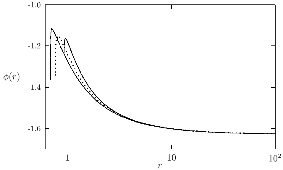
Figure 5: Dilaton field for the singular solution (66). Each curve corresponds to a different solution characterized by a different value of r_s ( r_s = 0.92, 0.75, 0.62 ).
