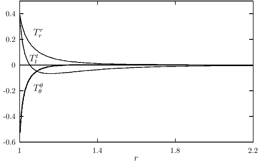
Figure 3: Components of the energy-momentum tensor for r_h = 1 black hole.
