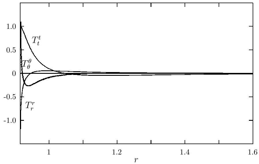
Figure 7: Components of the energy-momentum tensor for the r_s = 0.92 singular solution (66).
