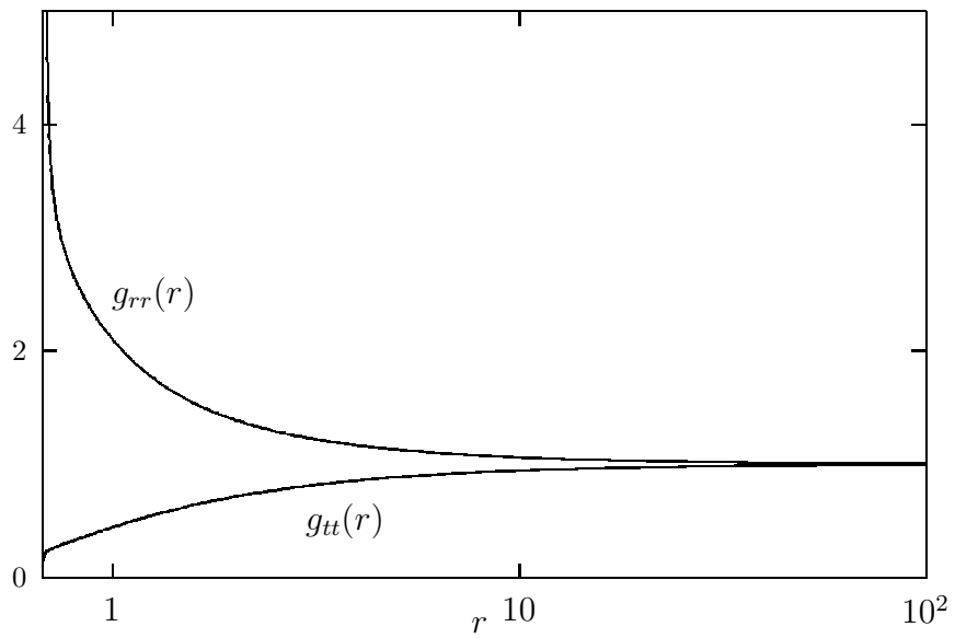
Figure 6: Metric components for the r_s = 0.68 singular solution (66).
